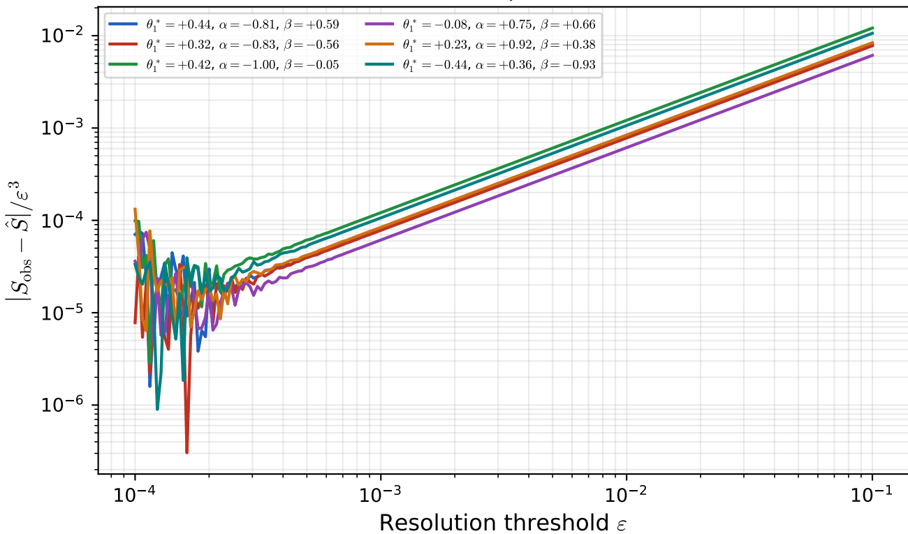
(b) Normalised remainder — O(\varepsilon^3) bound at \theta^* \neq 0 [Example 1]
