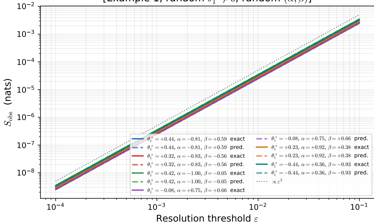
(a) Off-center check: S_{\text{obs}}^{\text{exact}} vs. \hat{S} = \frac{1}{2}\varepsilon^2 v^\top I(\theta^*) v [Example 1, random \theta_1^* \neq 0 , random (\alpha, \beta) ]
