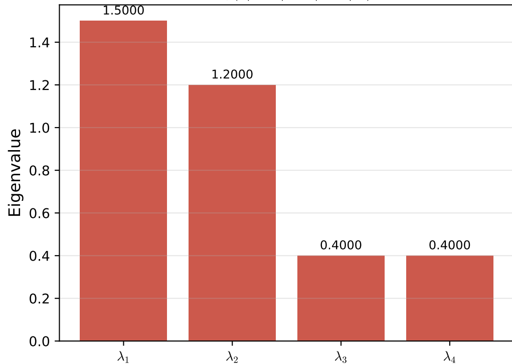
Example 2: I(\theta^*) eigenvalues
