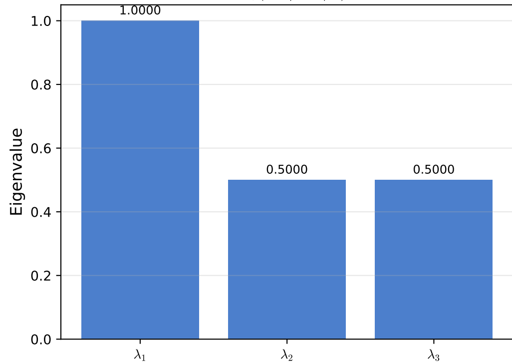
Example 1: I(\theta^*) eigenvalues
