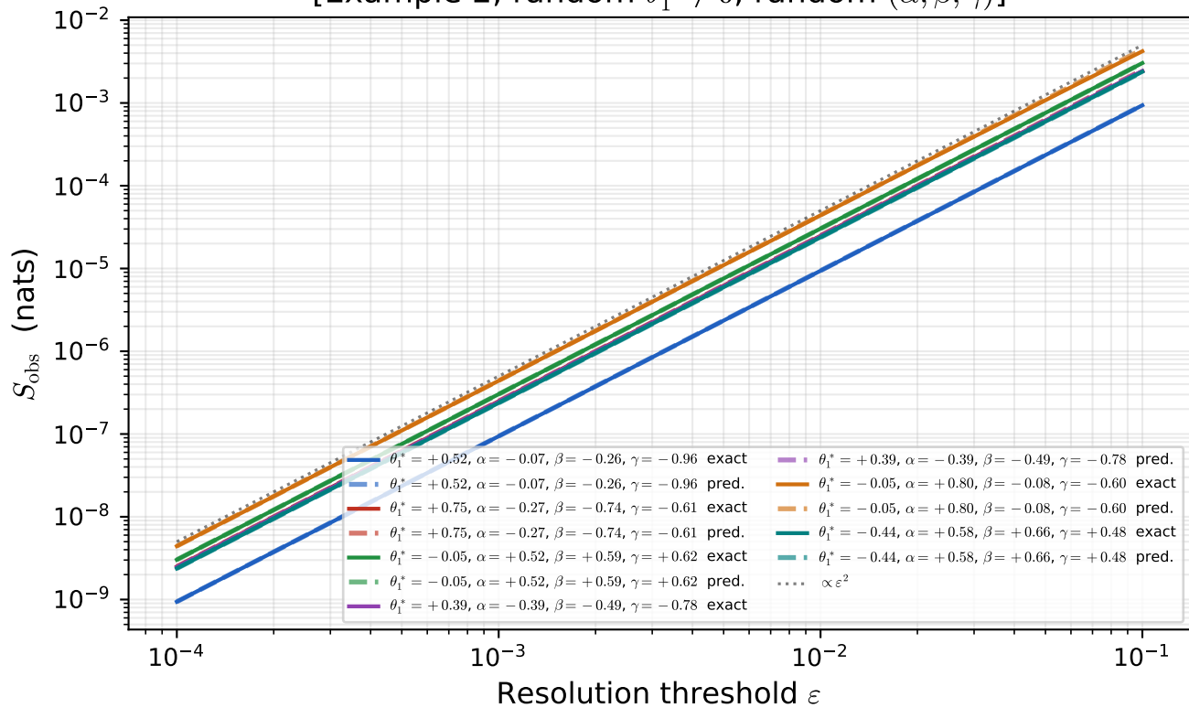
(a) Off-center check: S_{\text{obs}}^{\text{exact}} vs. \hat{S} = \frac{1}{2}\varepsilon^2 v^\top I(\theta^*)v [Example 2, random \theta_1^* \neq 0 , random (\alpha, \beta, \gamma) ]
