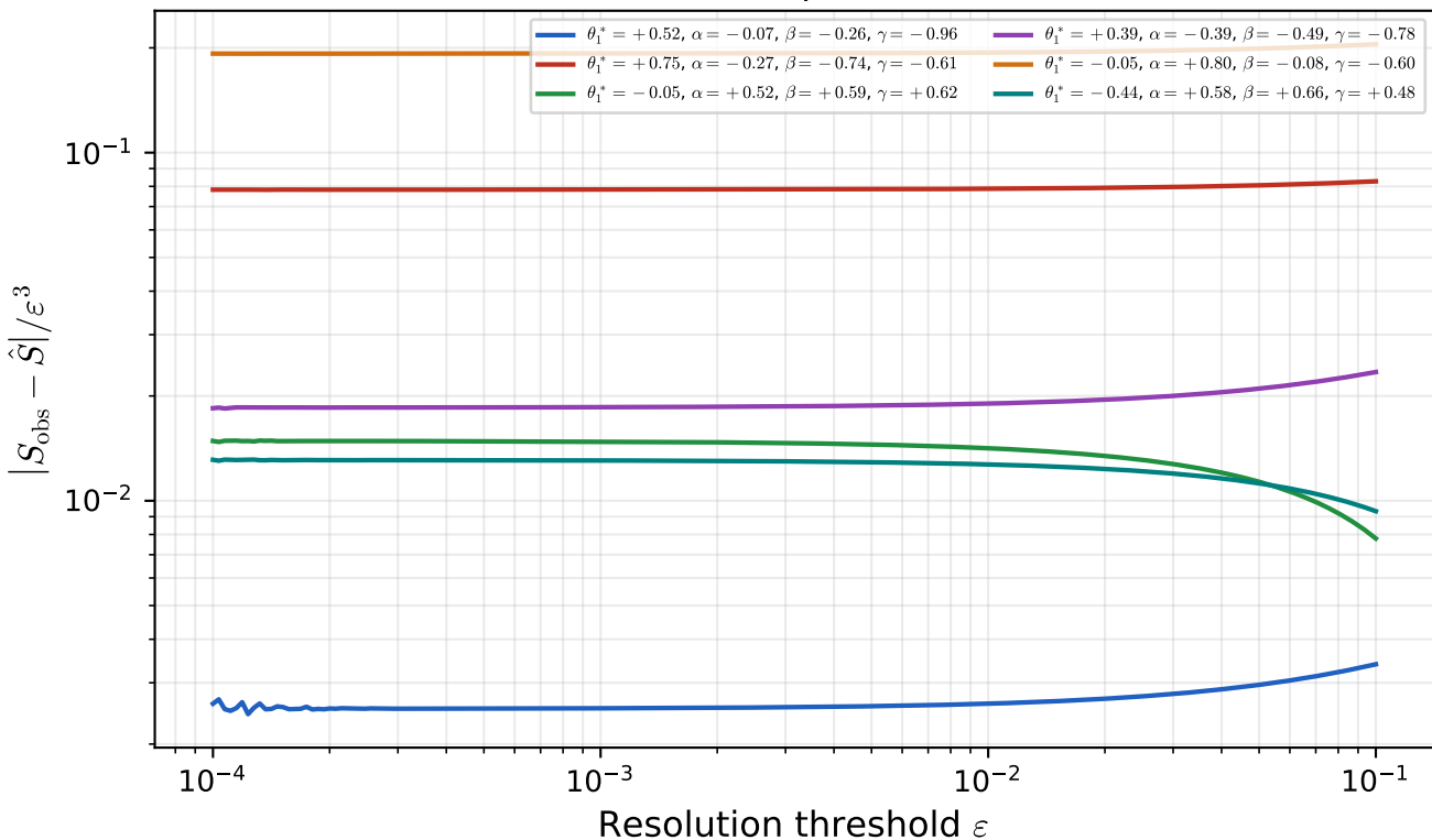
(b) Normalised remainder — O(\varepsilon^3) bound at \theta^* \neq 0 [Example 2]
