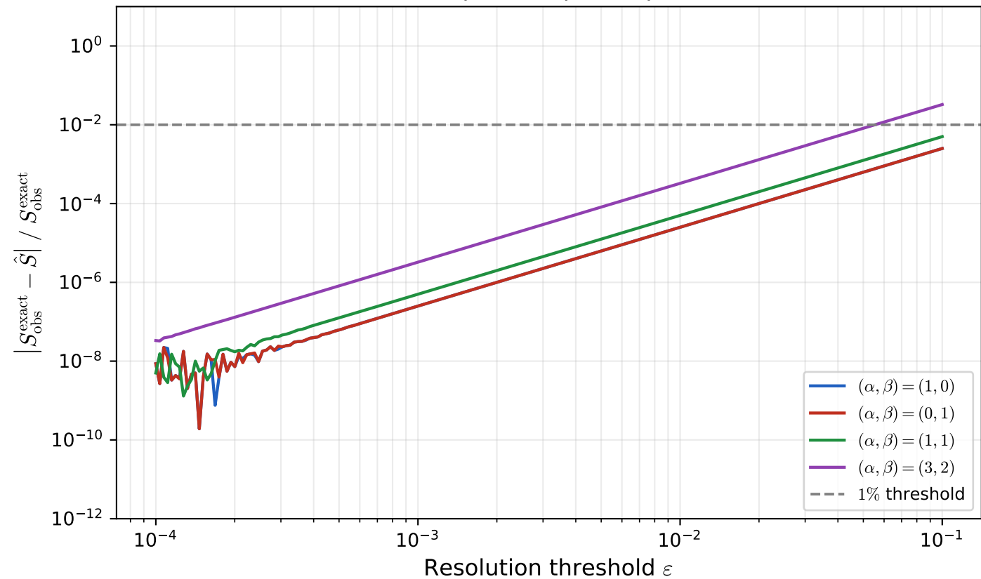
Relative error of quadratic approximation [Example 1: 4-point space]
