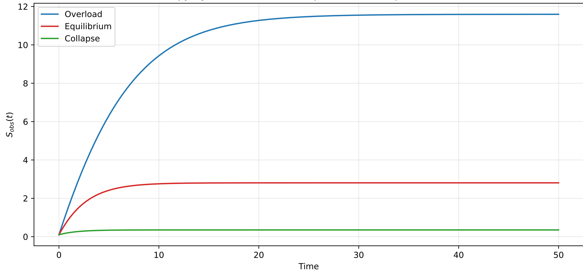
Entropy Dynamics: Overload / Equilibrium / Collapse (seed: 42)
