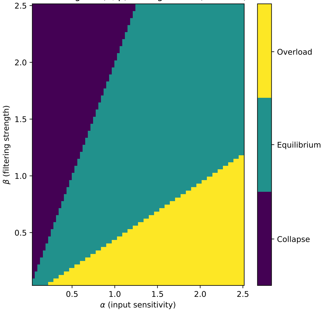
Phase diagram ( \alpha , \beta ) — long-time S (seed: 42)
