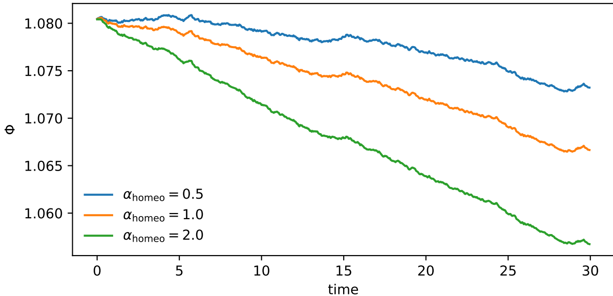
Effect of homeostatic strength on collective order
