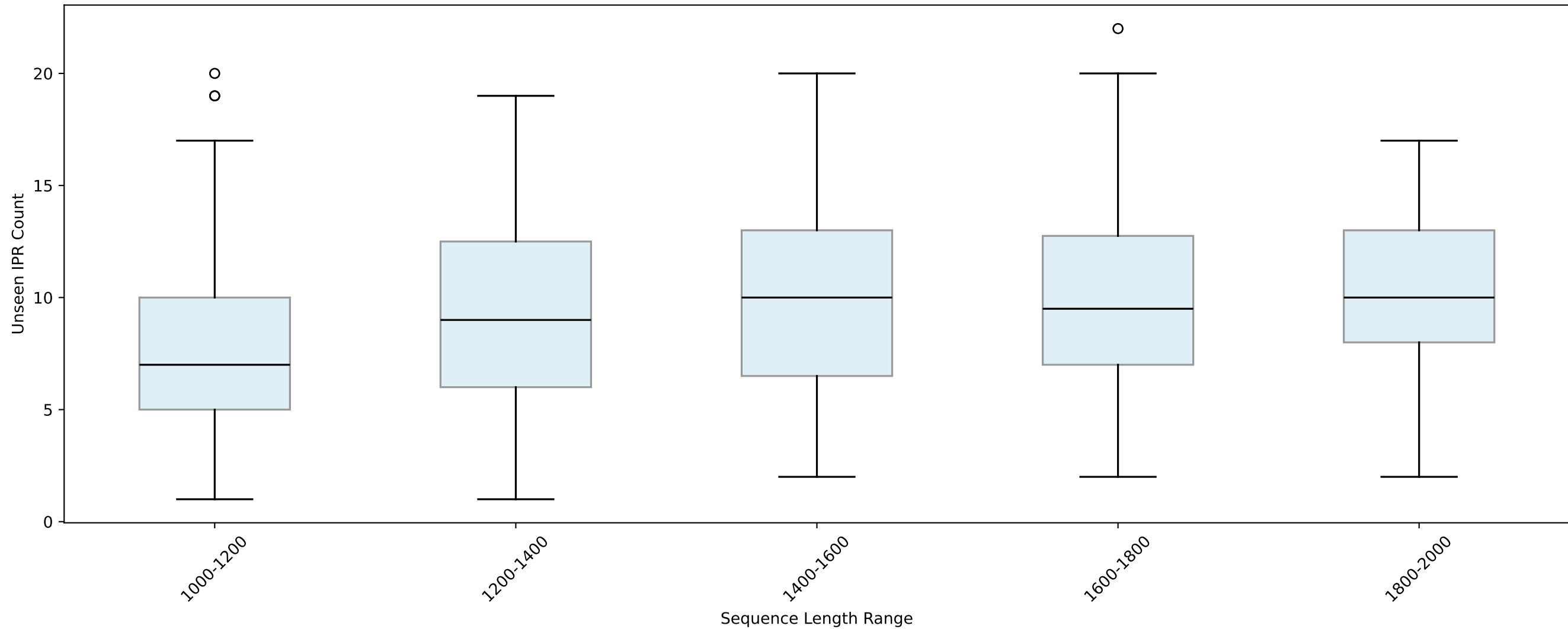
Unseen IPR Distribution per Length Range
