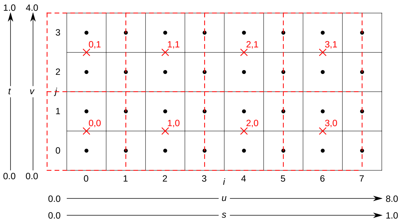
Figure 9. 420 downsampling, x\text{ChromaOffset}=\text{COSITED\_EVEN} , y\text{ChromaOffset}=\text{MIDPOINT}
