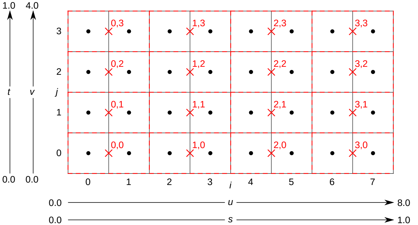
Figure 6. 422 downsampling, xChromaOffset=MIDPOINT
