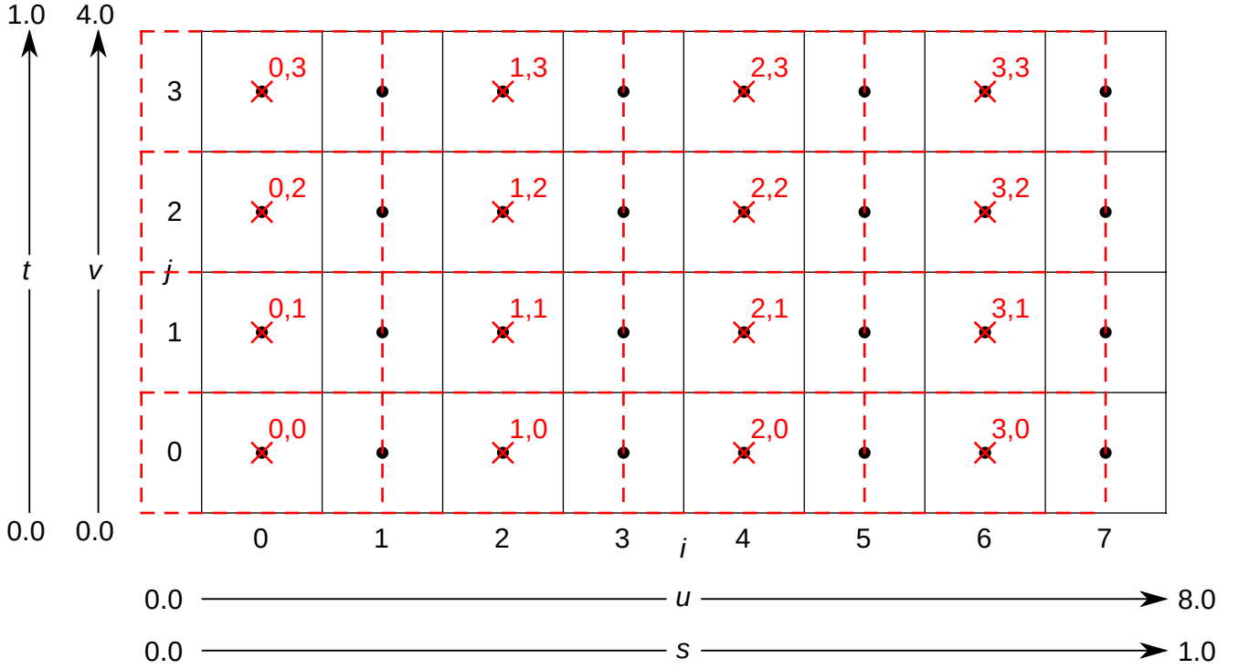
Figure 5. 422 downsampling, xChromaOffset=COSITED\_EVEN
