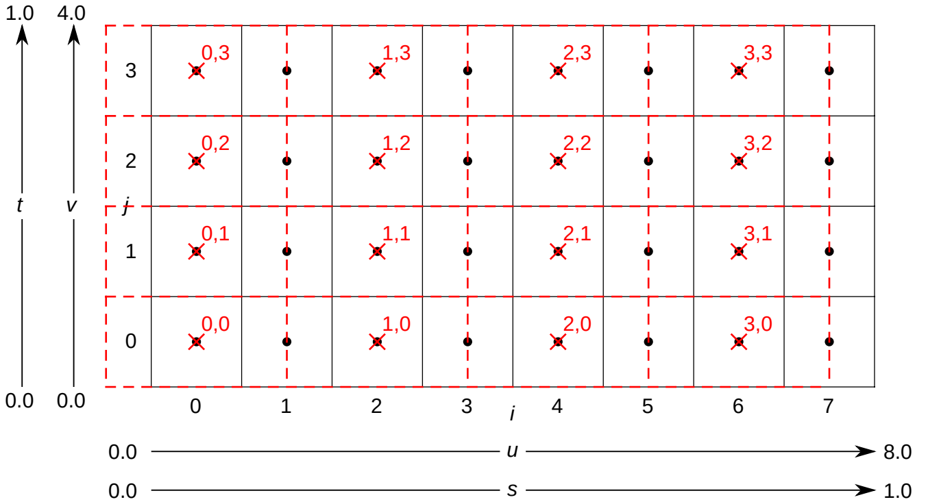
Figure 5. 422 downsampling, xChromaOffset=COSITED\_EVEN
