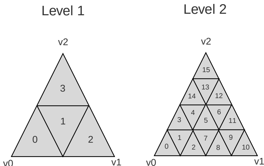
Figure 29. Example ordering for micromap data
