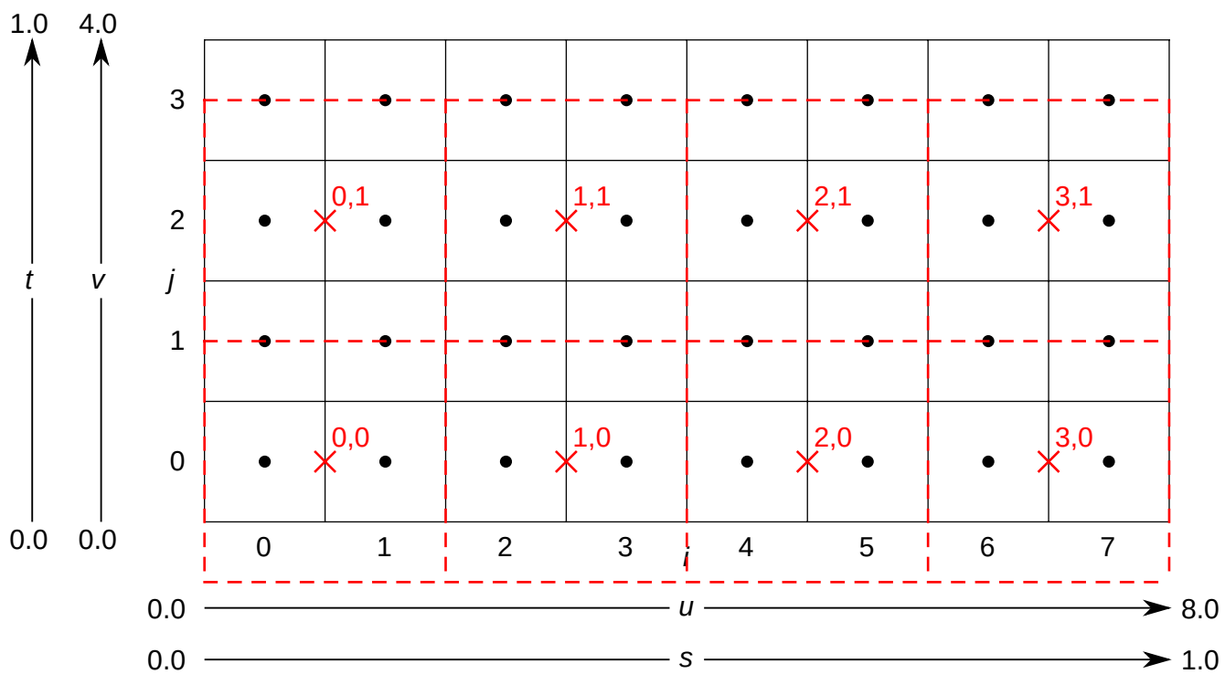
Figure 9. 420 downsampling, xChromaOffset=MIDPOINT , yChromaOffset=COSITED\_EVEN
