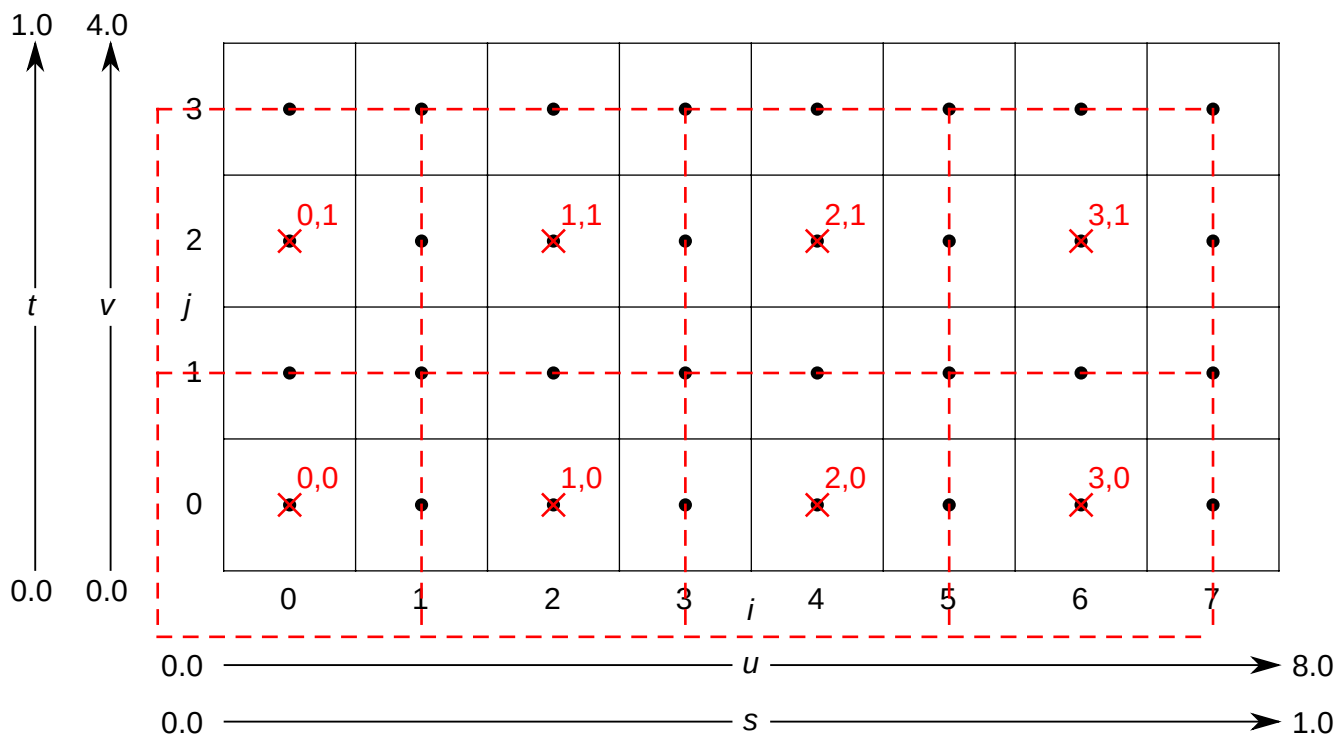
Figure 8. 420 downsampling, xChromaOffset=COSITED\_EVEN , yChromaOffset=COSITED\_EVEN
