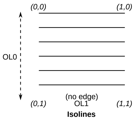
Figure 15. Domain parameterization for tessellation primitive modes (upper-left origin)
