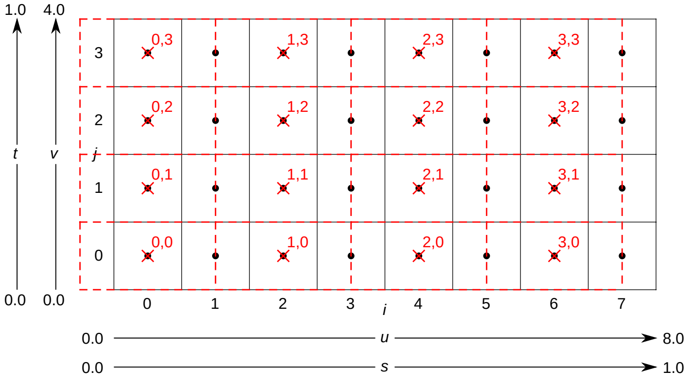
Figure 5. 422 downsampling, xChromaOffset=COSITED\_EVEN
