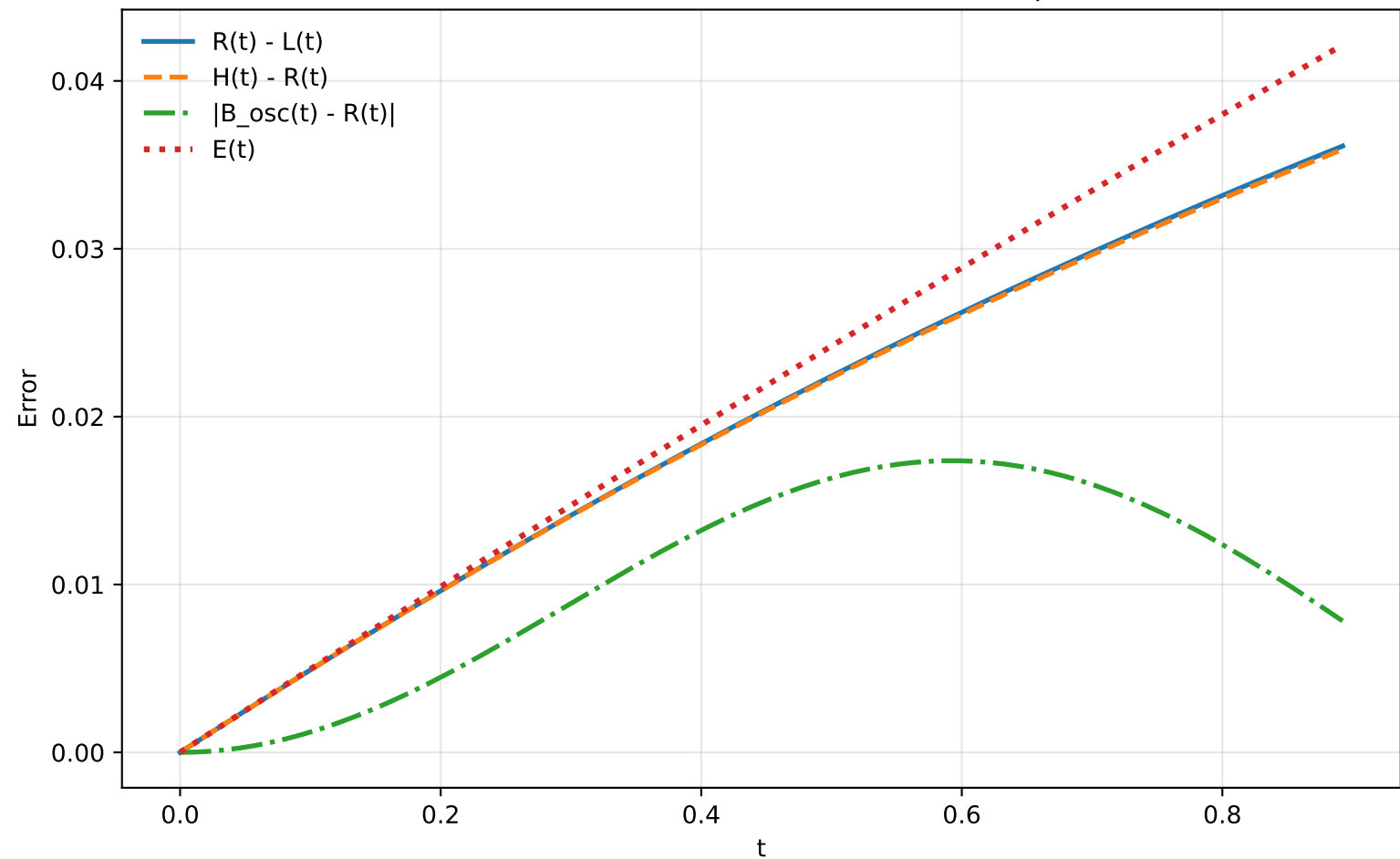
Numerical errors and theoretical envelope
