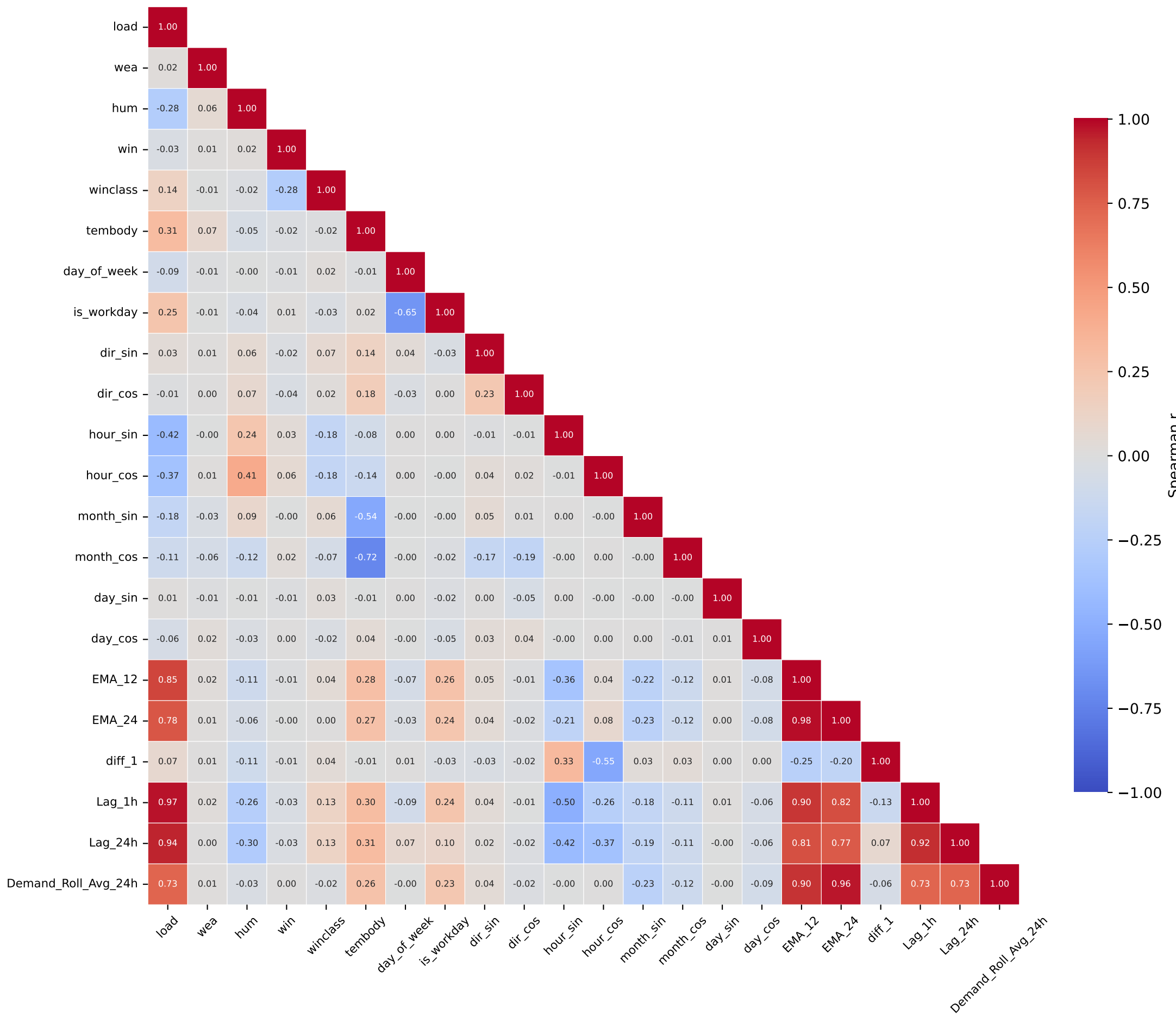
SH — Spearman Correlation
