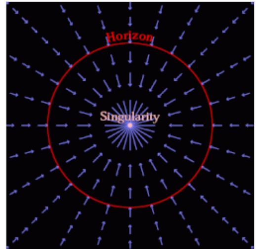
Picture of space falling into a Schwarzschild black hole at the Newtonian escape speed. Outside the horizon (red), the infalling speed is less than the speed of light; inside it is greater. At the event horizon, the infalling speed equals the speed of light. [6] Credit: Andrew Hamilton, JILA
