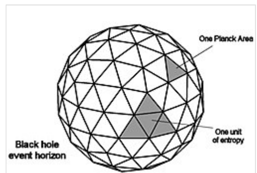
Diagram by Jacob Bekenstein of the entropy on a black hole's event horizon.
