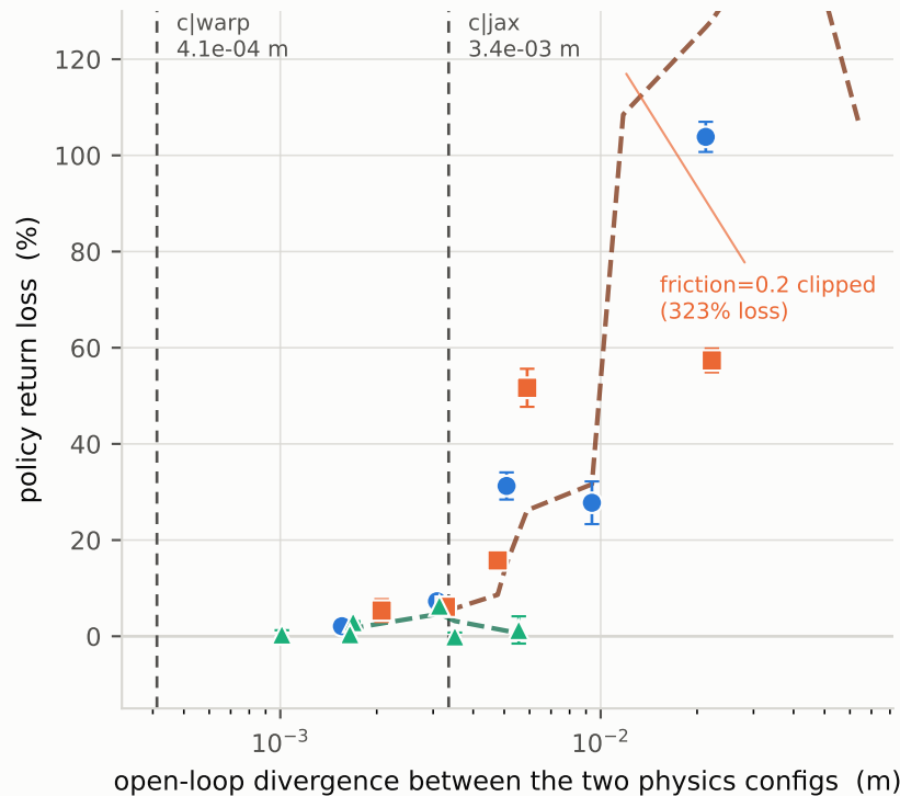
Return loss (one point clipped)
