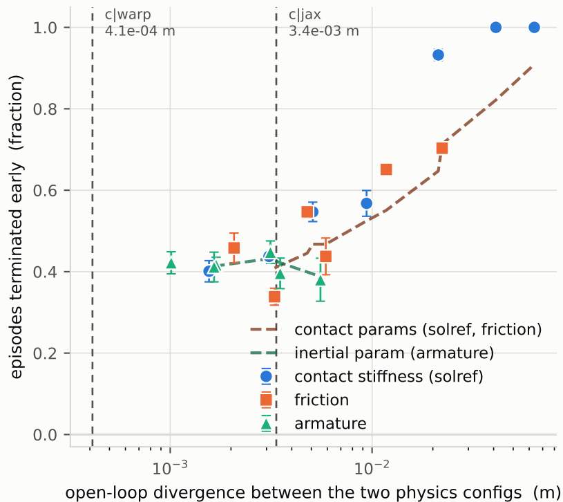
Contact mismatch &gt;&gt; inertial mismatch, at equal divergence
