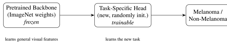
Figure 2.3: The transfer-learning recipe used throughout this report: a frozen, ImageNet-pretrained backbone (CNN or ViT) acts as a general-purpose feature extractor, feeding into a small trainable head adapted to the skin-cancer classification task.
