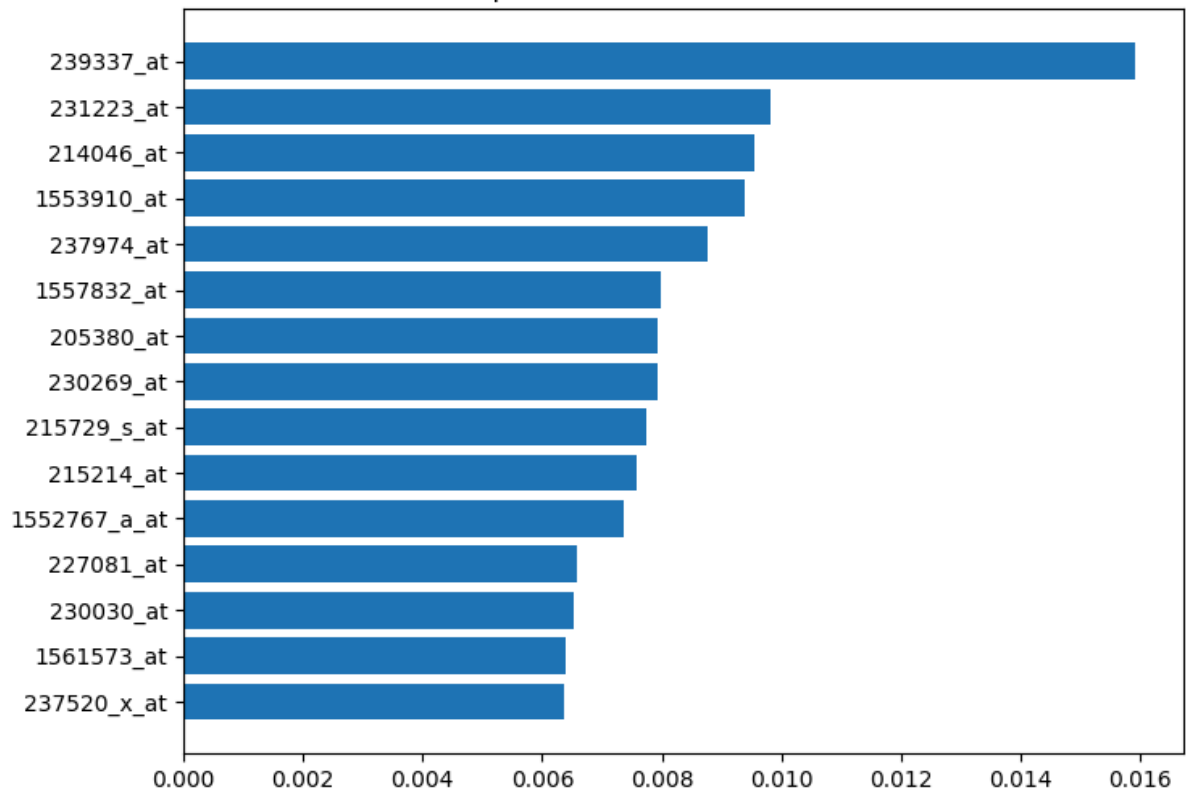
Top 15 Features - Random Forest
