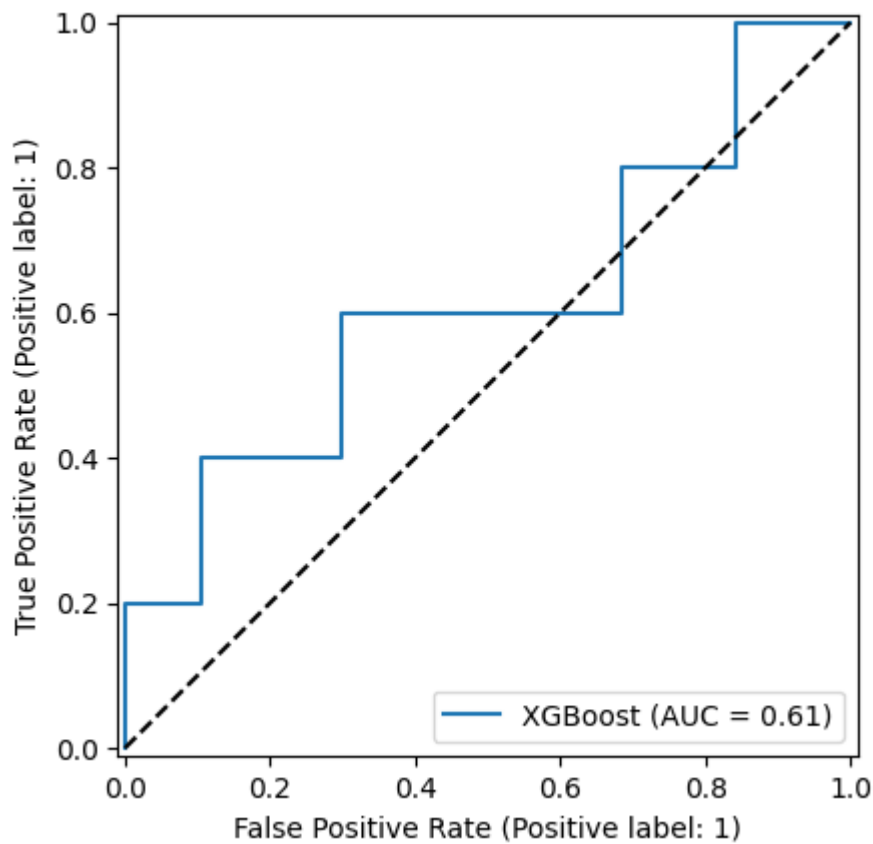
ROC Curve - XGBoost
