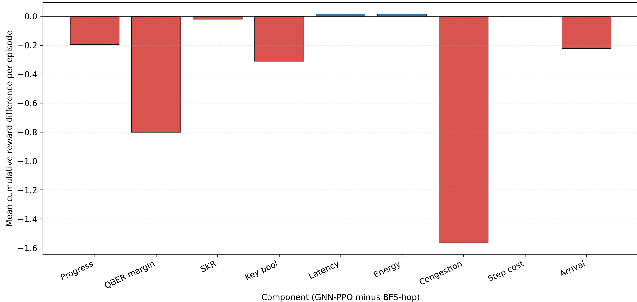
Paired reward-component difference: GNN-PPO – BFS-hop
