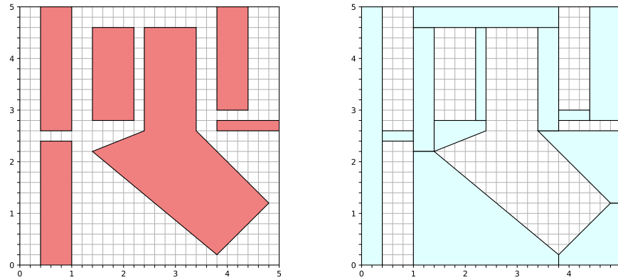
Figure 6.9 - Left : A simple 2D configuration-space with obstacles in red. Right : A convex decomposition of the collision-free configuration space.
