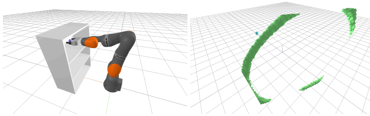
Figure 6.5 - The image on the right is a visualization of the "grasp the sphere" constraint in configuration space -- the x,y,z, axes in the visualizer correspond to the three joint angles of the planarized iiwa.
