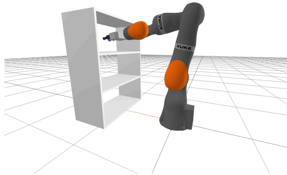
Figure 6.2 - A richer inverse kinematics problem: solve for the joint angles, q , that allow the robot to reach into the shelf and grab the object, while avoiding collisions.
