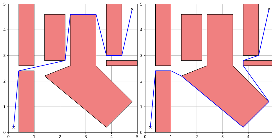
Figure 6.10 - Left : The GcsTrajOpt solution with a minimum-distance cost. Right : The GcsTrajOpt solution with a minimum-time cost (and
