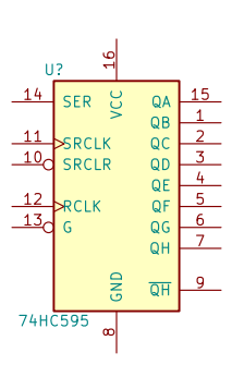
74HC595
