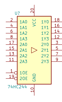
74HC244
