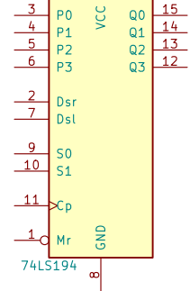
74LS194
