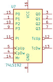
74LS192
