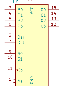
74LS194
