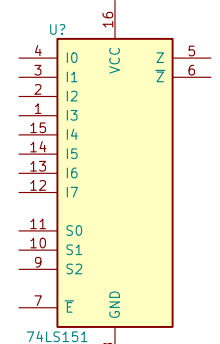
74LS151
