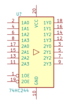
74HC244
