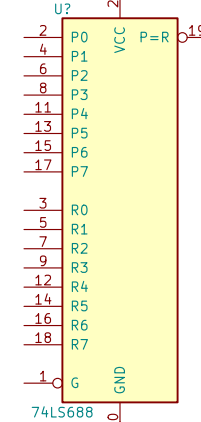
74LS688
