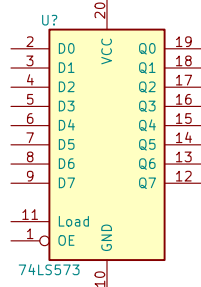
74LS573
