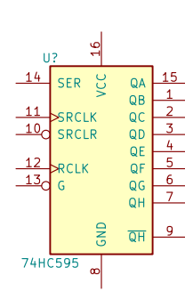
74HC595
