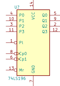
74LS196
