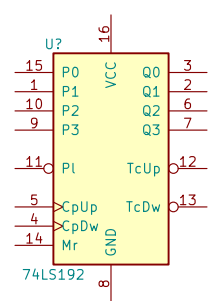
74LS192
