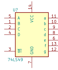
74LS49
