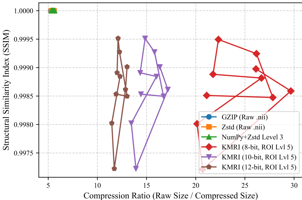
Rate-Distortion Performance: SSIM
