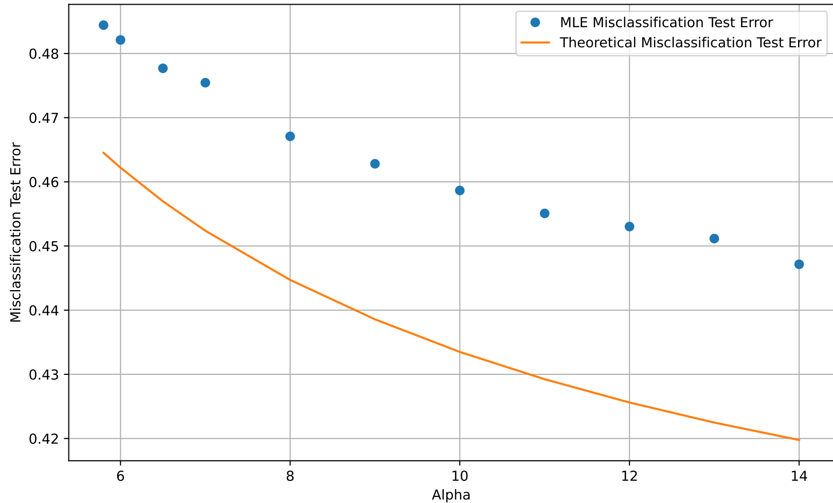
MLE vs Theoretical Misclassification Test Error
