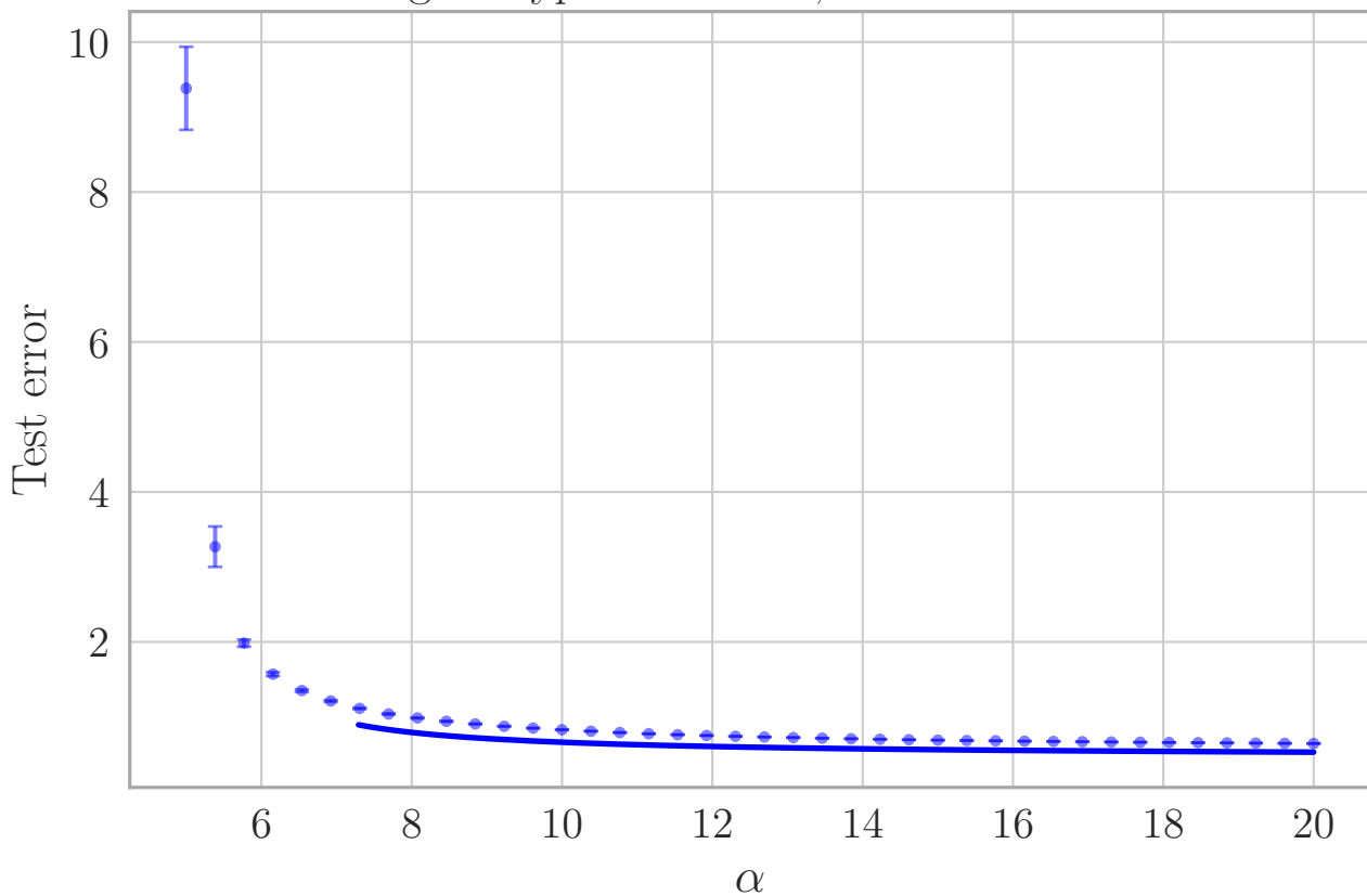
Tangent hyperbolic with, 500 hidden units
