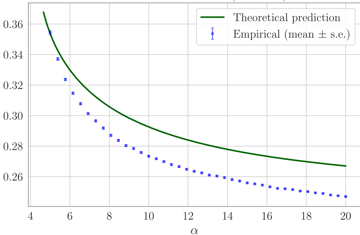
Random ReLU Features (350 units)
