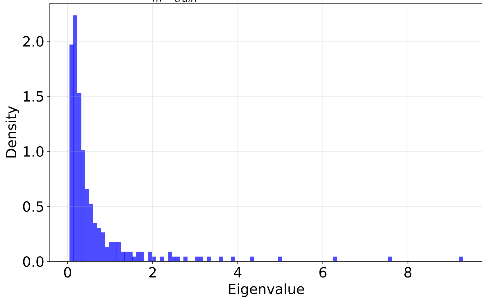
ESD of \frac{1}{m}H_{train}^T H_{train} (full 250 features after relu)
