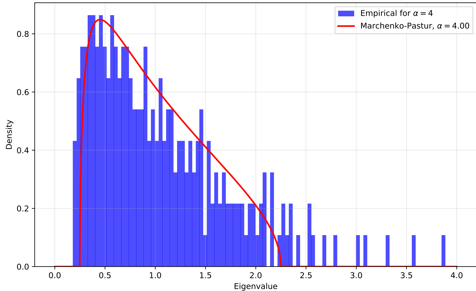
ESD of \frac{1}{m}H^TH from subsample of 1000
