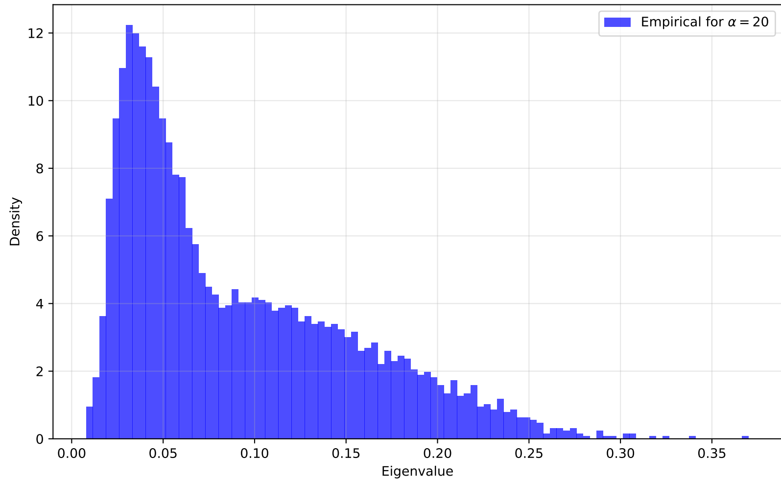
ESD of Hessian
