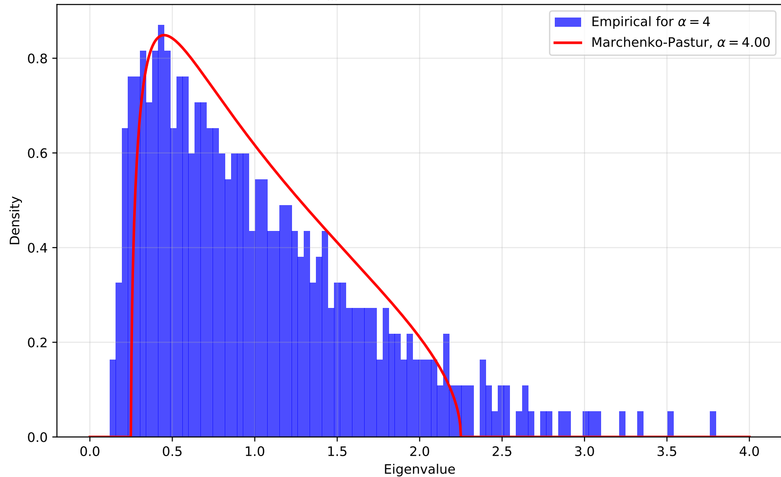
ESD of \frac{1}{m}H^TH from subsample of 2000
