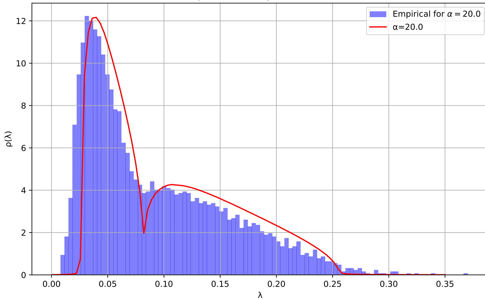
Spectral Density for \alpha=20.0
