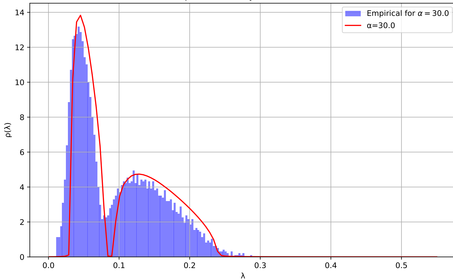
Spectral Density for \alpha=30.0
