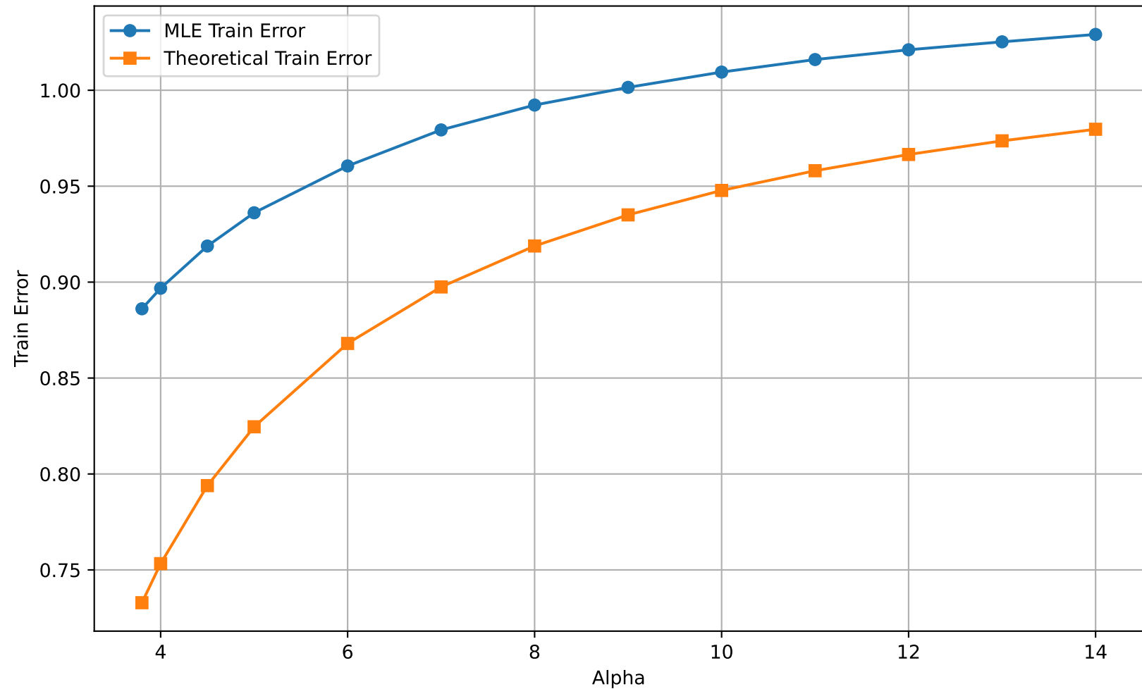
MLE vs Theoretical Train Error
