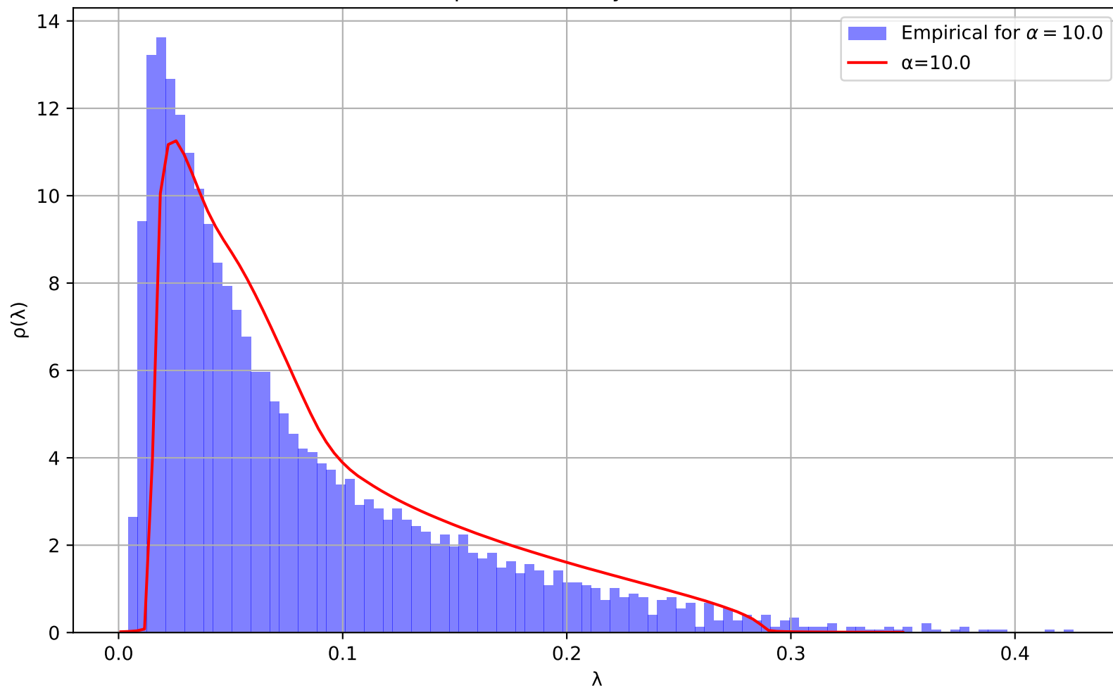
Spectral Density for \alpha=10.0
