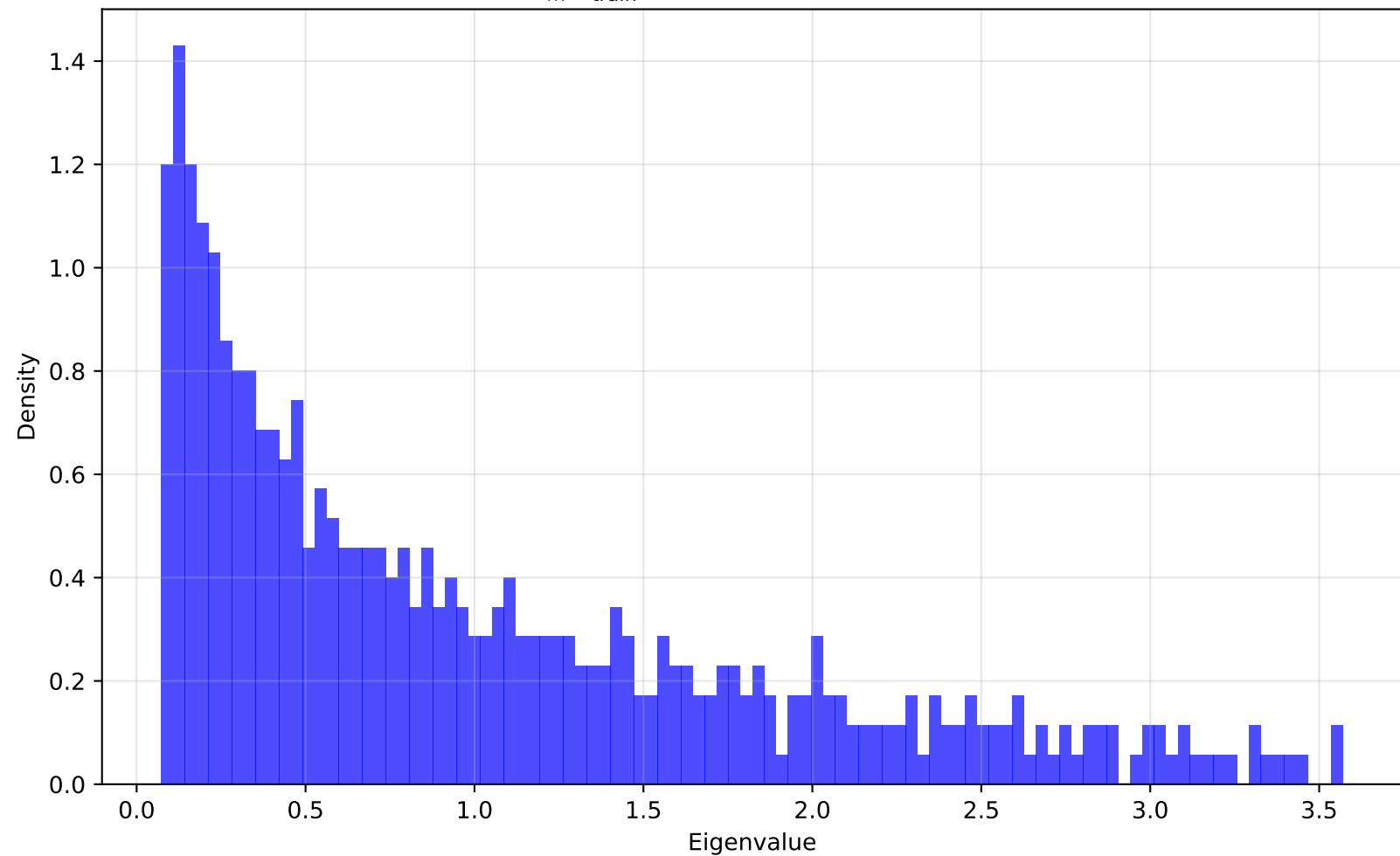
ESD of \frac{1}{m}\hat{H}_{\text{train}}^T\hat{H}_{\text{train}} from subsample of 2000
