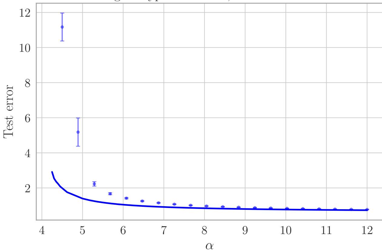
Tangent hyperbolic with, 250 hidden units
