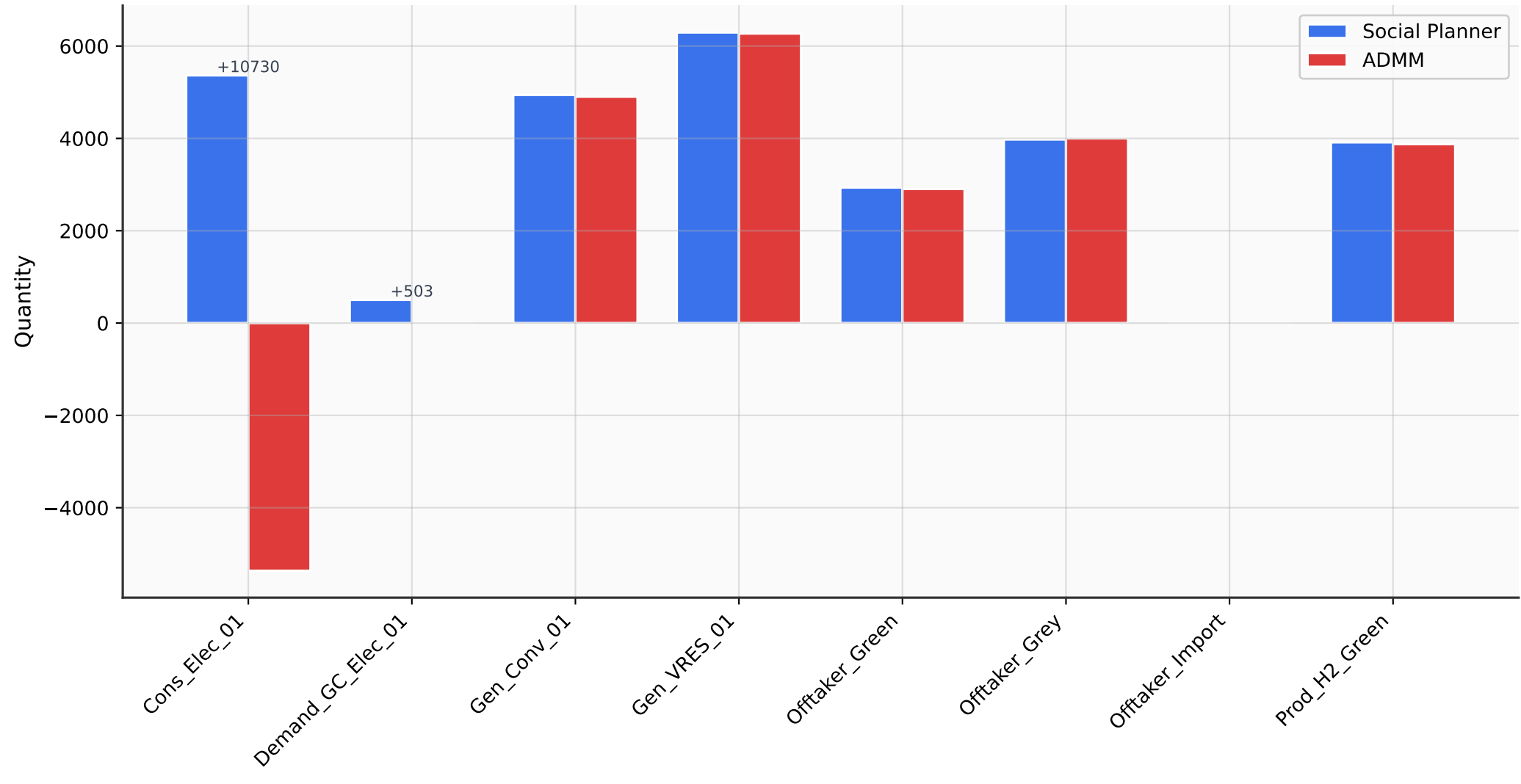
Agent quantities: Social Planner vs ADMM
