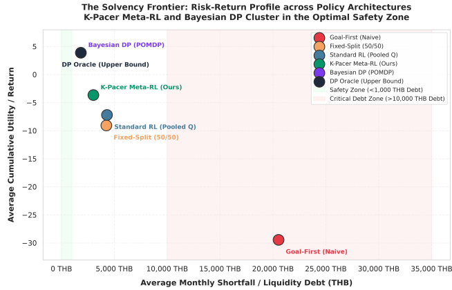
Fig. 3. Example reward versus shortfall-risk frontier used for policy comparison.
