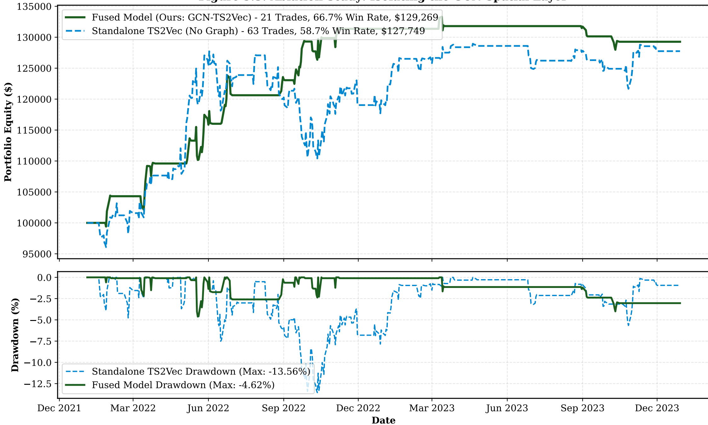
Figure 5.3: Ablation Study: Isolating the GCN Spatial Layer
