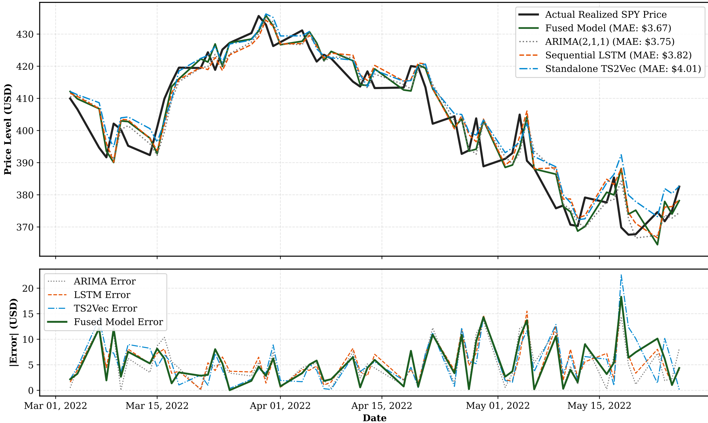
Figure 5.4: Model Price Forecasting and Daily Error Comparison Across Representative Window
