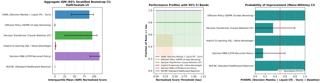
Figure 1: RLiabale Statistical Evaluation on HalfCheetah-v5 showing Probability of Improvement and Aggregate IQM with 95% Stratified Bootstrap Confidence Intervals.
