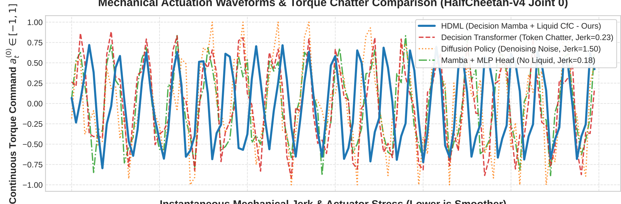
Instantaneous Mechanical Jerk & Actuator Stress (Lower is Smoother)
