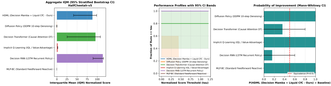
Figure 1: RLiabe Statistical Evaluation on HalfCheetah-v5 showing Probability of Improvement and Aggregate IQM with 95% Stratified Bootstrap Confidence Intervals.
