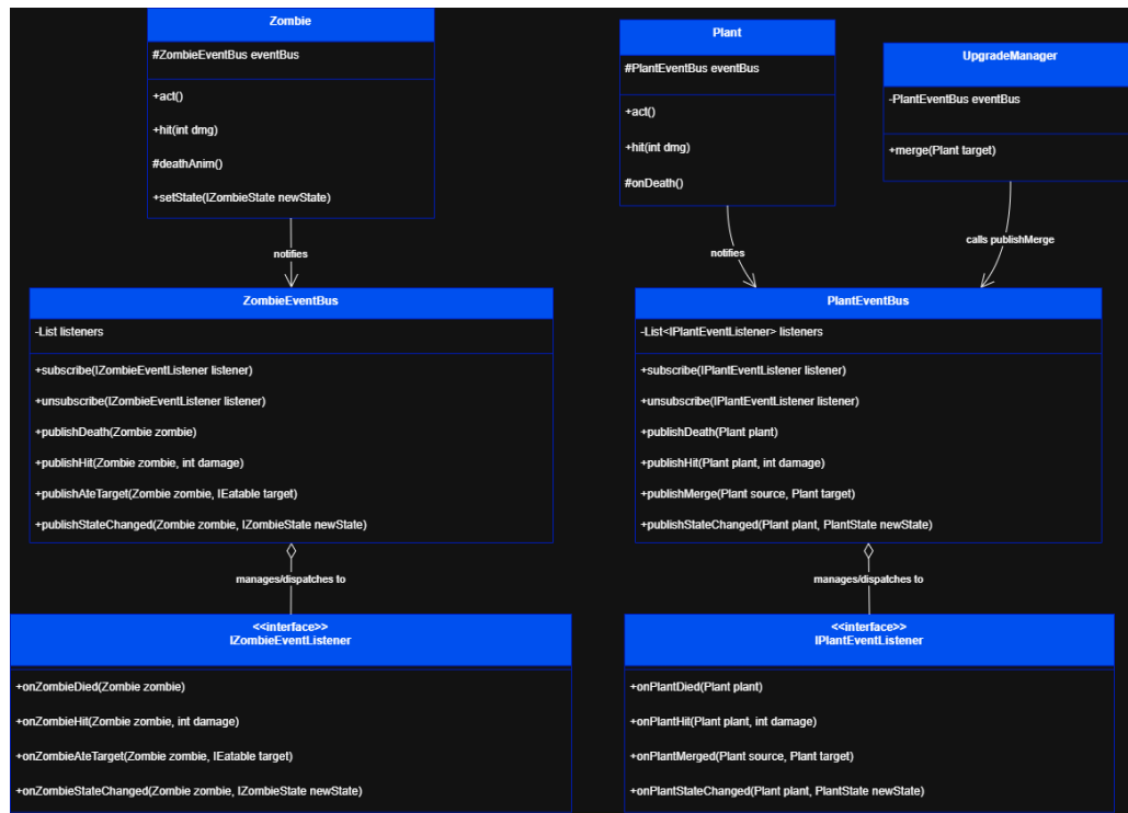
Figure 19: Event Bus architecture decoupling the connection between the Subject and system Subscribers.
