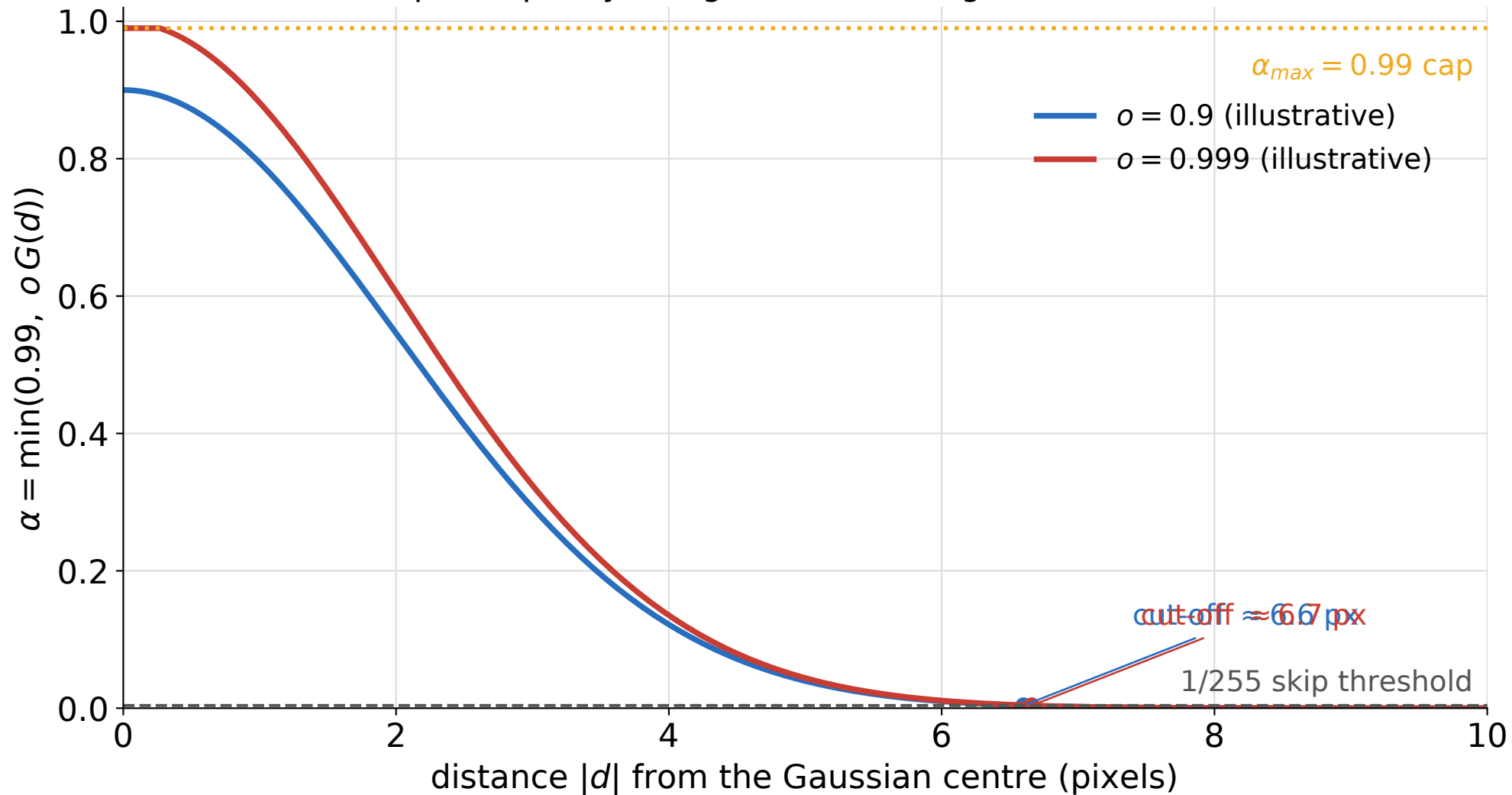
Per-pixel opacity along a line, \Sigma' = \text{diag}(4, 4) , illustrative
