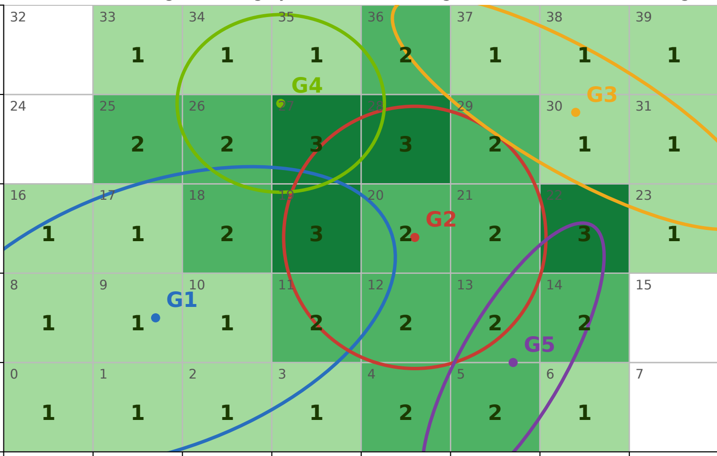
Illustrative 8 x 5 tile grid. Small grey number: tile id. Large number: Gaussians touching the tile
