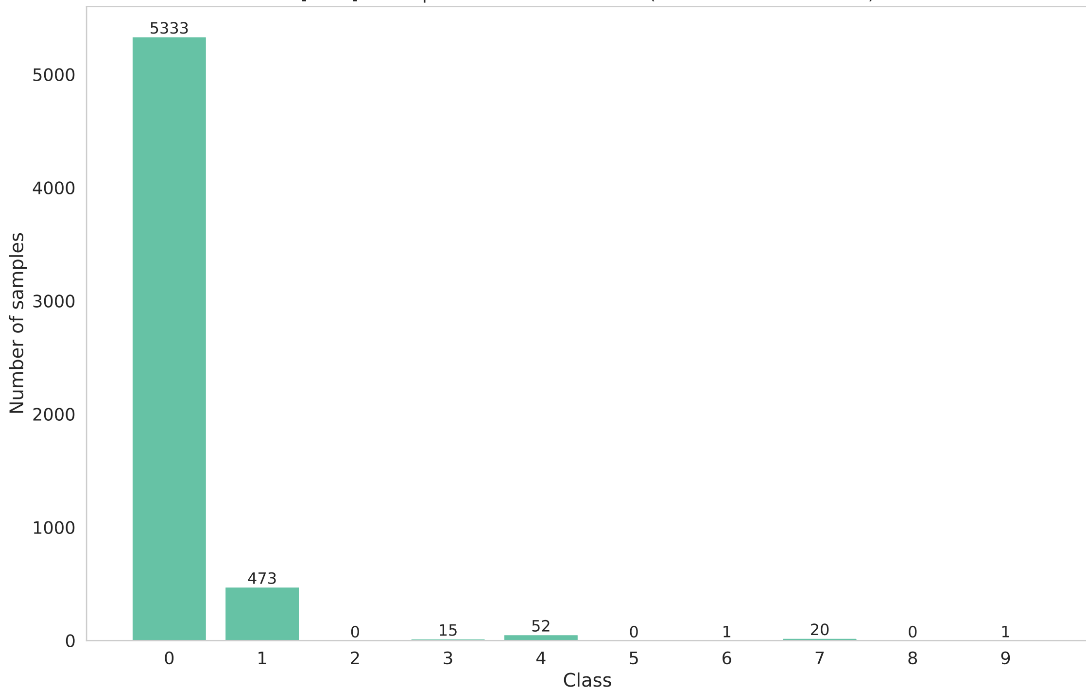
[train] Participant 5 data distribution (Non-IID - dirichlet - 0.1)
