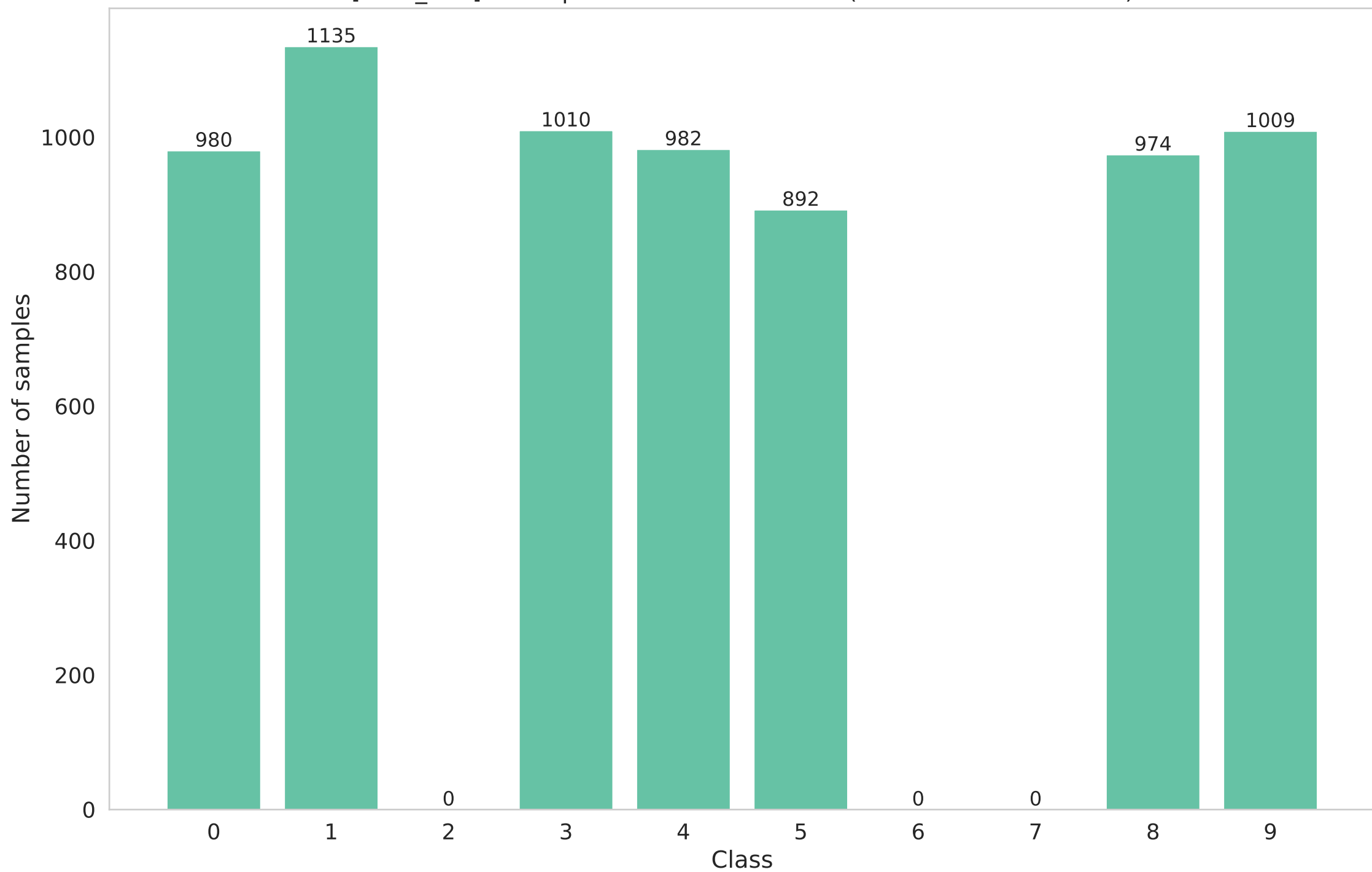
[local_test] Participant 2 data distribution (Non-IID - dirichlet - 0.1)
