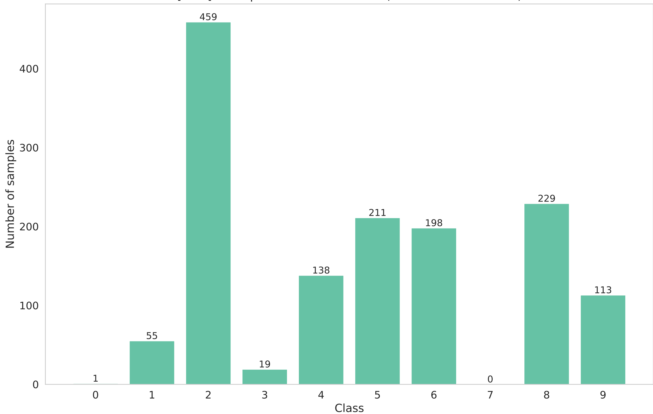
[train] Participant 0 data distribution (Non-IID - dirichlet - 0.5)
