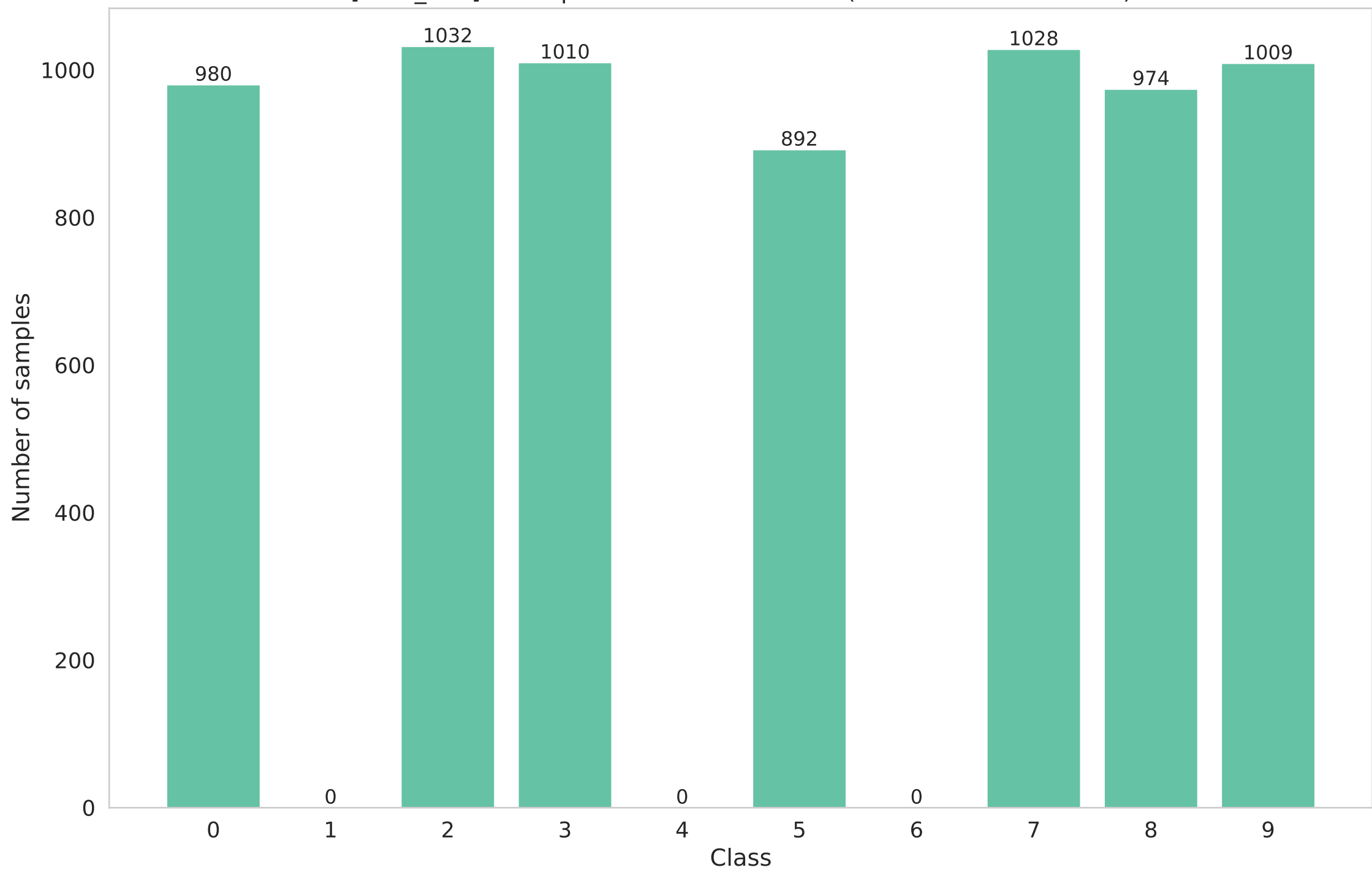
[local_test] Participant 0 data distribution (Non-IID - dirichlet - 0.1)
