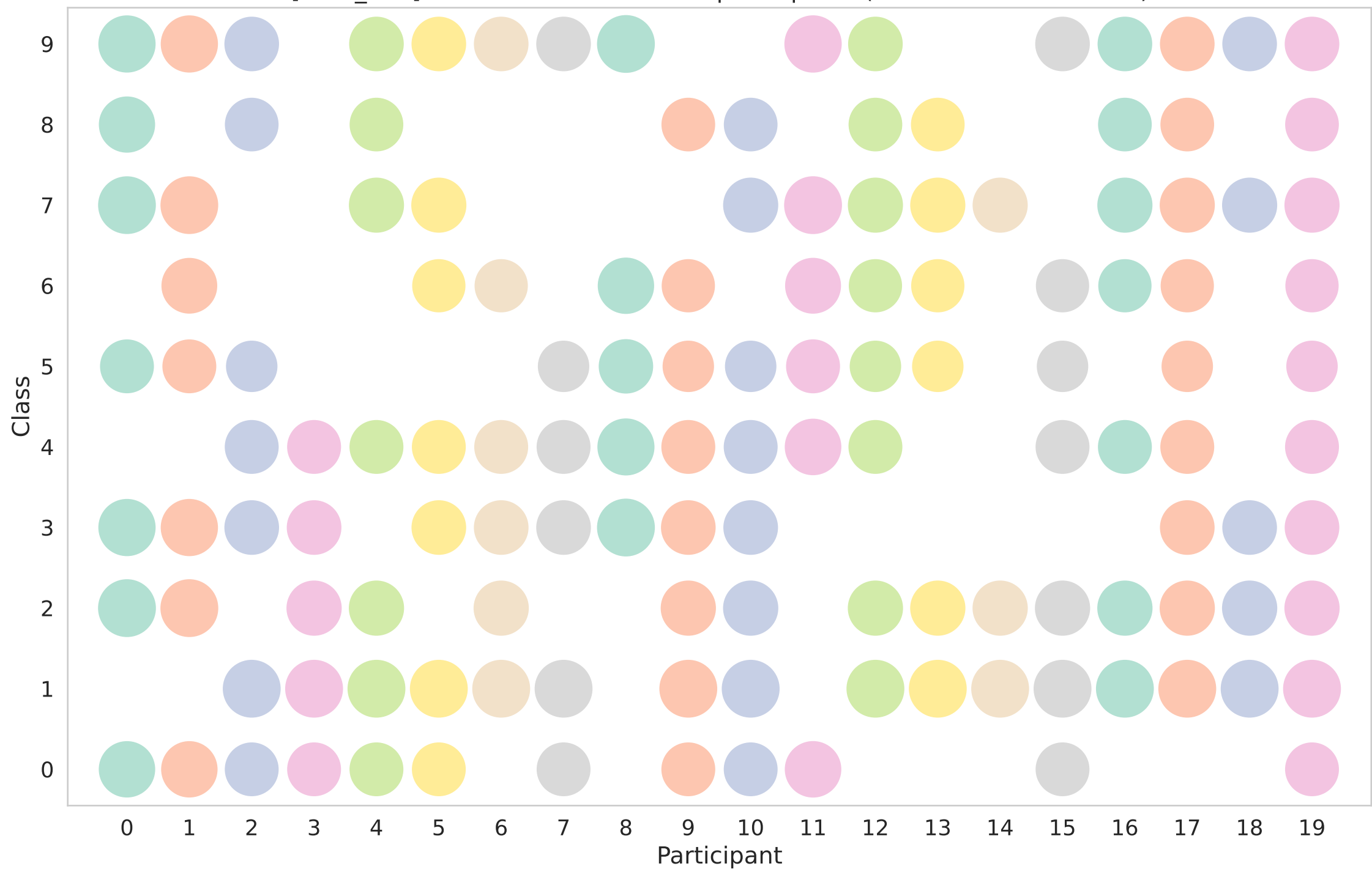
[local_test] Data distribution across participants (Non-IID - dirichlet - 0.1)
