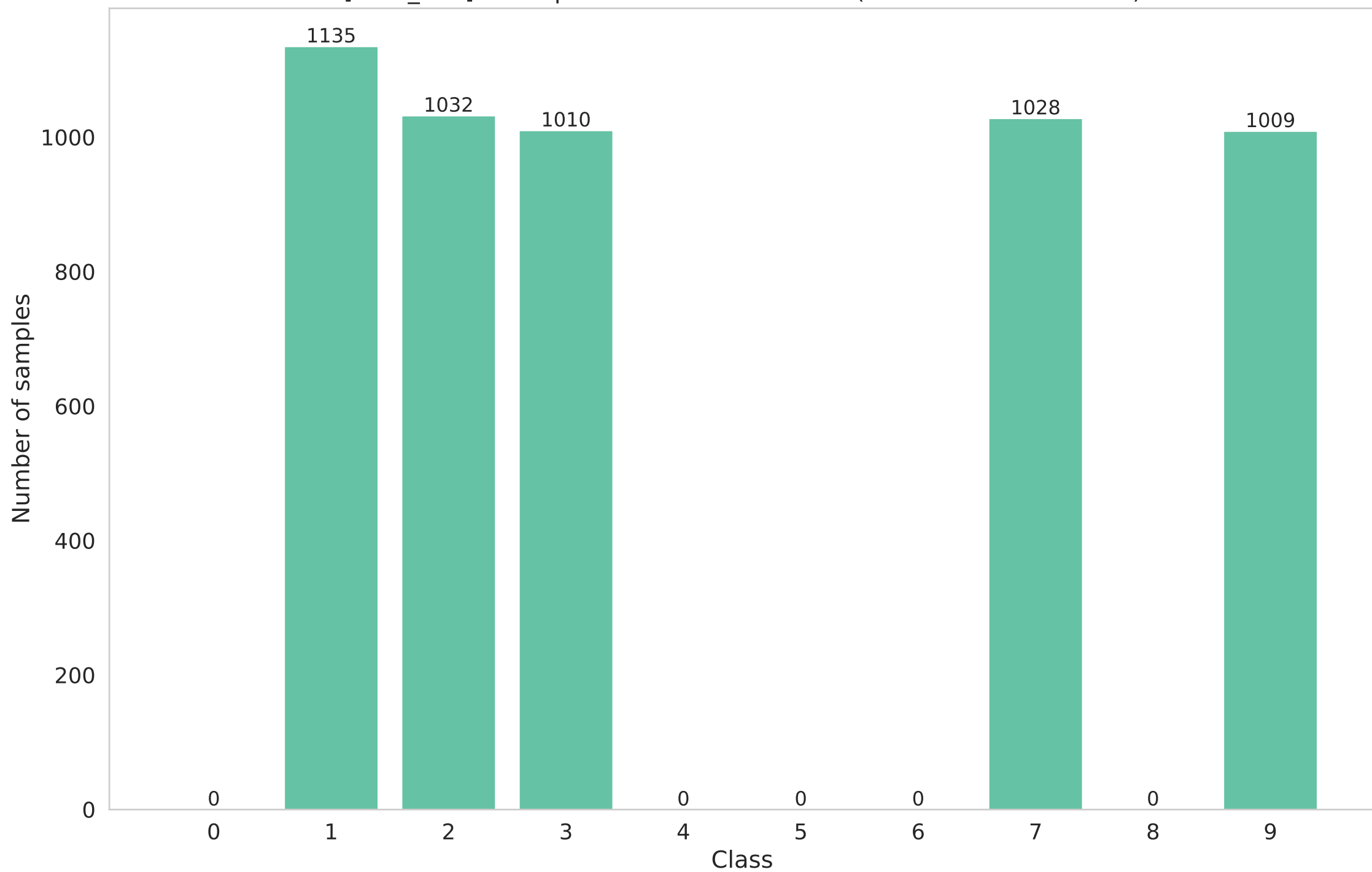
[local_test] Participant 18 data distribution (Non-IID - dirichlet - 0.1)
