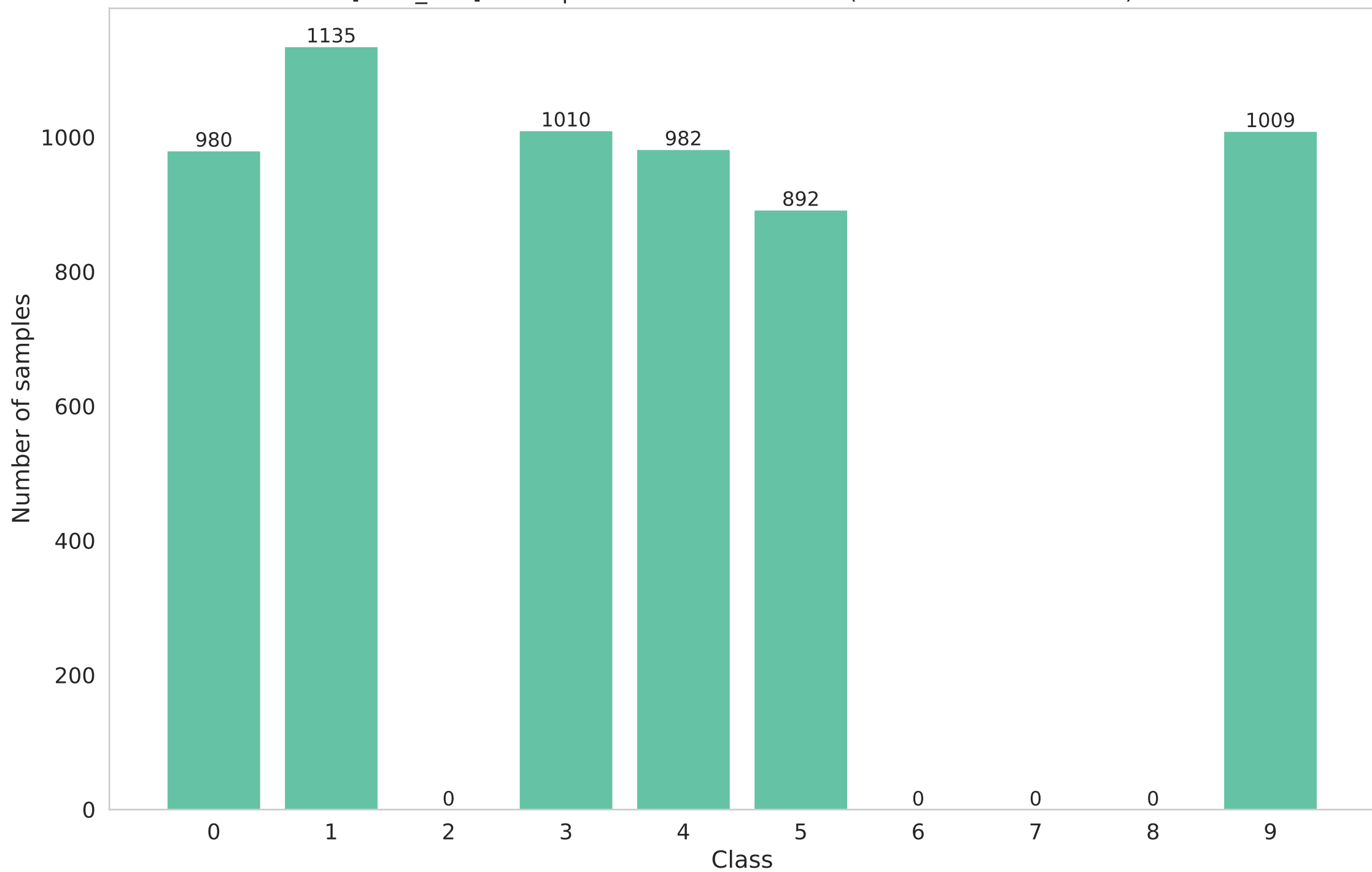
[local_test] Participant 7 data distribution (Non-IID - dirichlet - 0.1)
