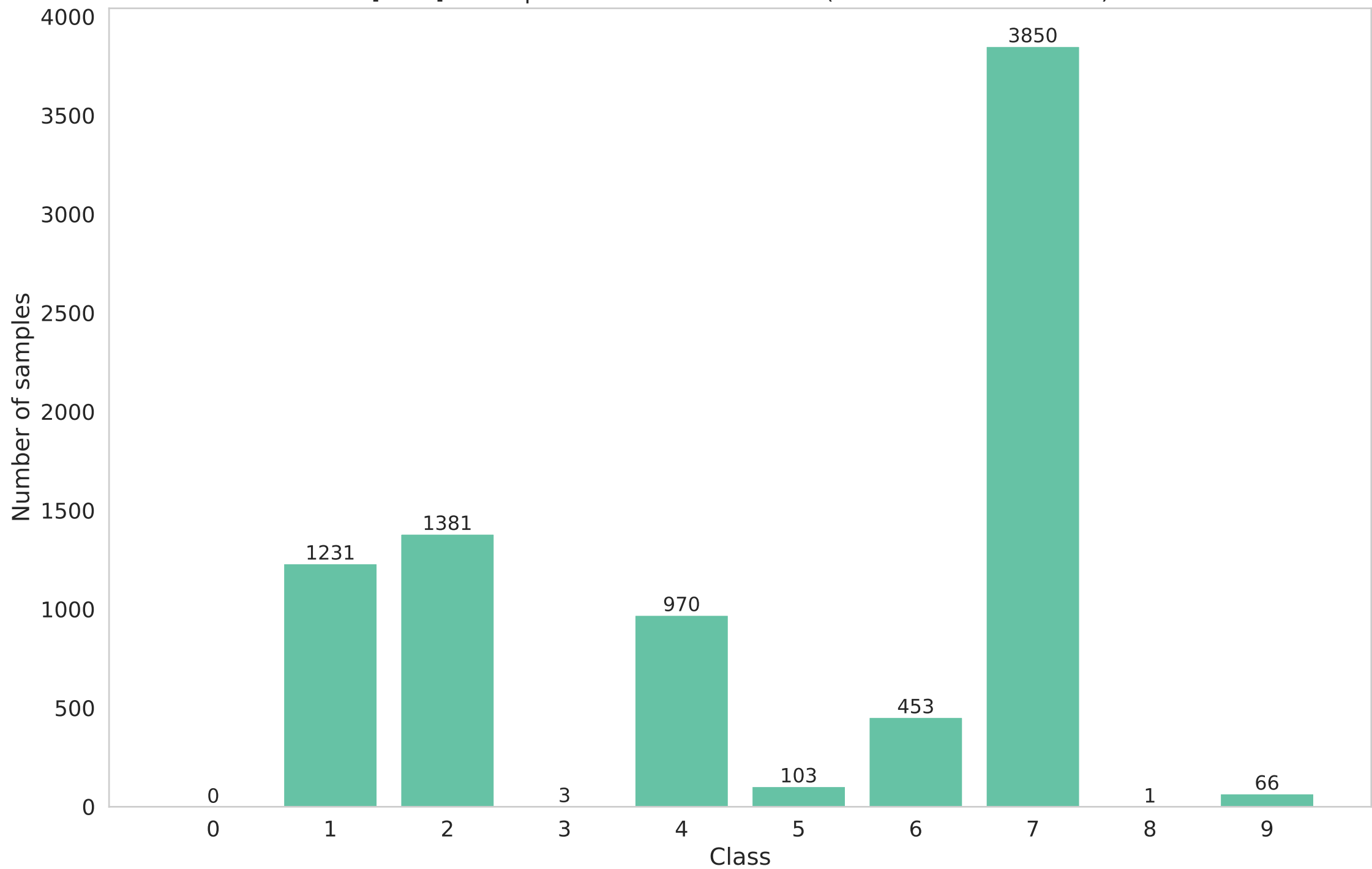
[train] Participant 17 data distribution (Non-IID - dirichlet - 0.1)
