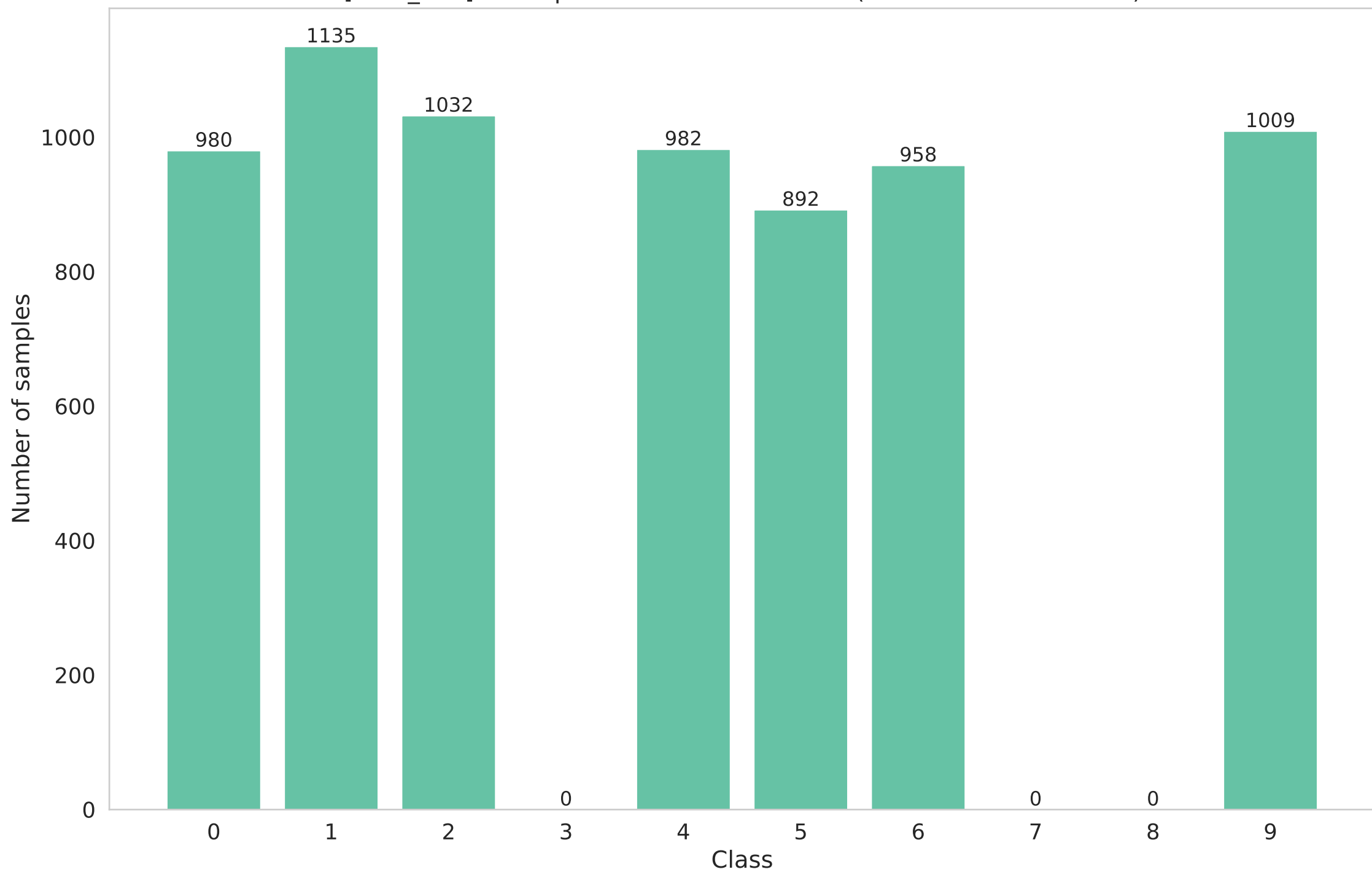
[local_test] Participant 15 data distribution (Non-IID - dirichlet - 0.1)
