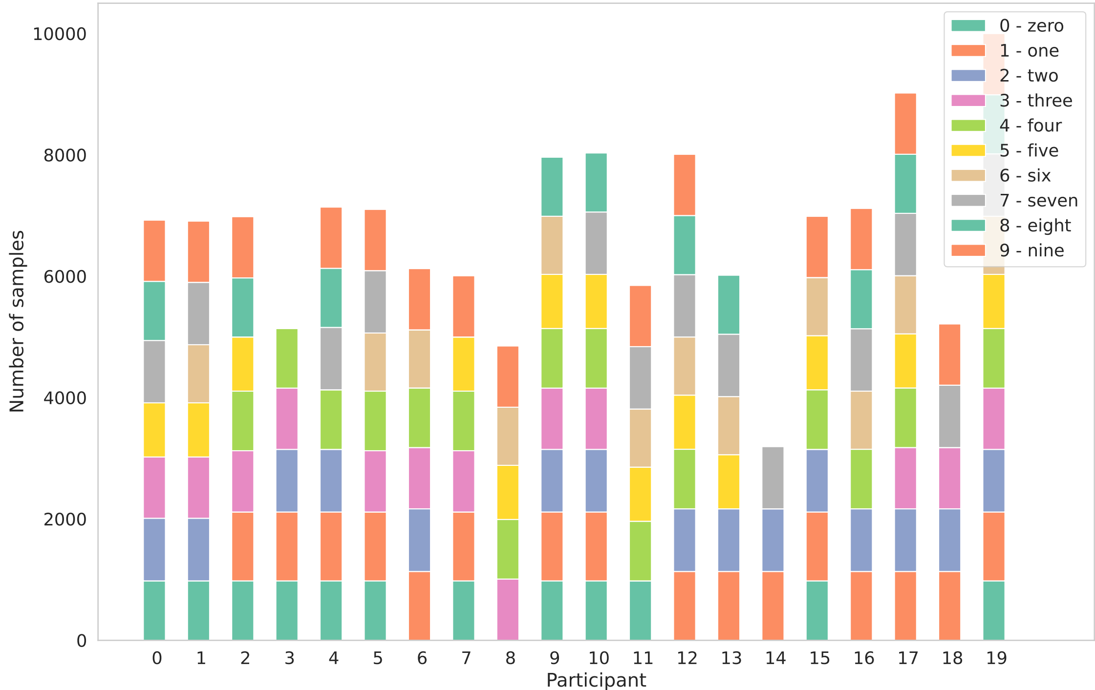
[local_test] Distribution of splitted datasets
