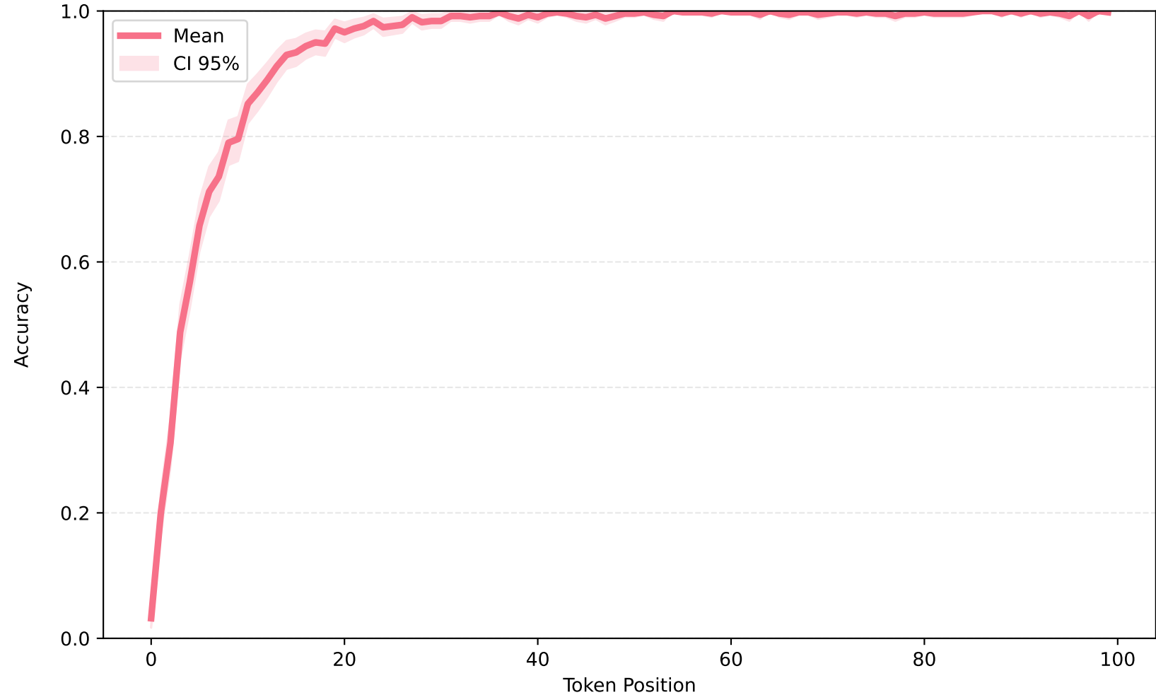
Accuracy per timestep
