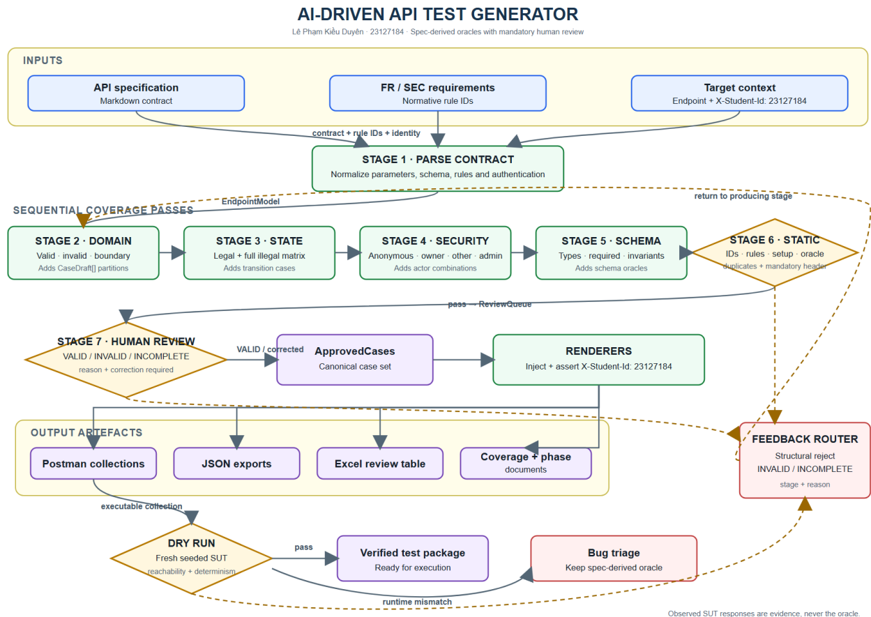
AI-driven API test generator pipeline
